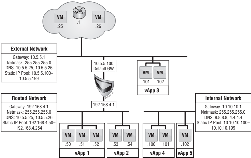
FIGURE 12.29 A direct vApp network consumes ports and IP addresses on the organization network it's connected to.
