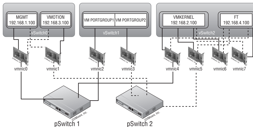
FIGURE 5.15 A configuration with eight NICs provides both redundancy and scalability.
