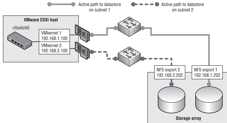
FIGURE 5.9 Without link aggregation, NFS redundancy requires multiple datastores and multiple VMkernel interfaces.
