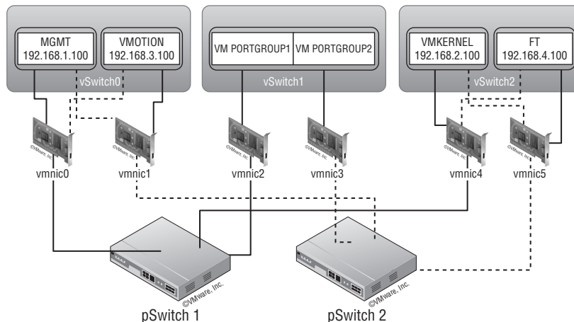
FIGURE 5.14 A six-NIC configuration provides redundancy for all components.
