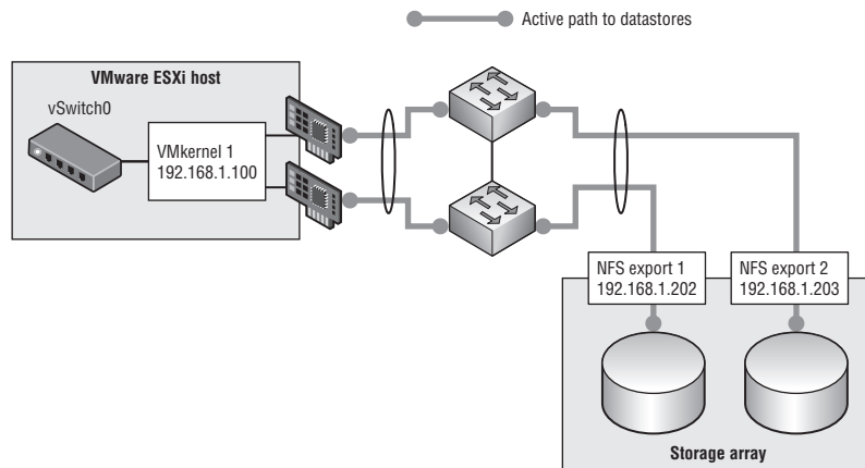
FIGURE 5.8 This configuration uses link aggregation for both the ESXi host and the storage array.
