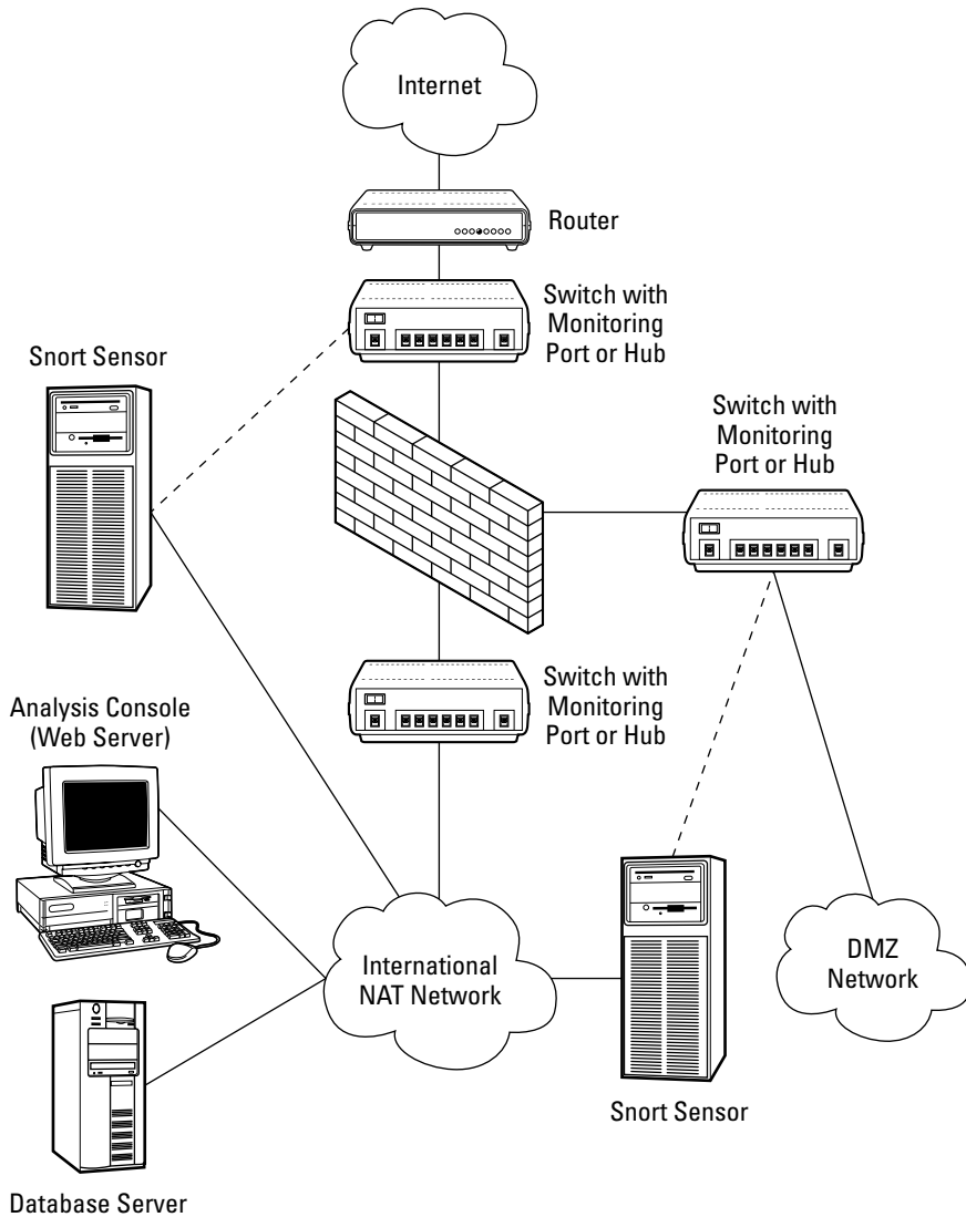
Figure 2-2: Additional Snort sensors monitoring separate subnets.
