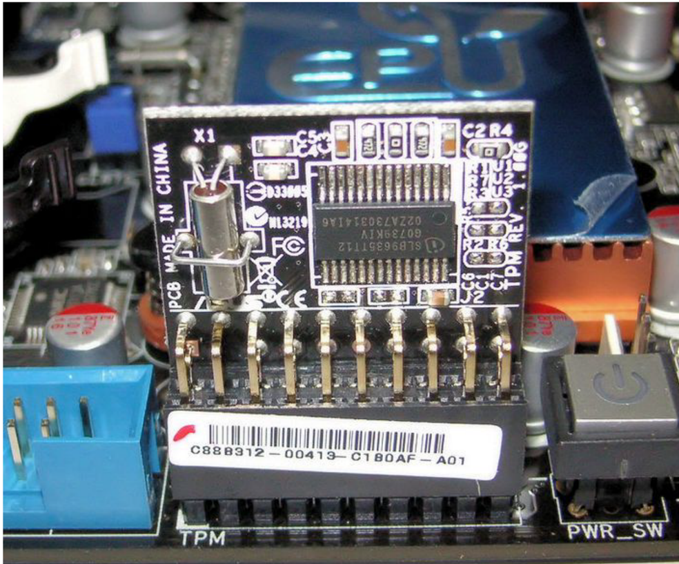
Figure 13.3 A chip implementing the TPM 2.0 standard, plugged into a motherboard. This chip can be called by the system's motherboard components as well as user applications running on the computer's OS. Photo from Wikipedia ( http://mng.bz/Q2je ).
