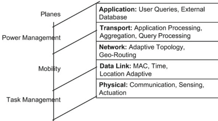
Fig. 20.2 Sensor network protocol stack
