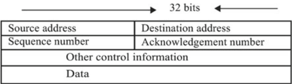
Fig. 1.19 TCP data structure
