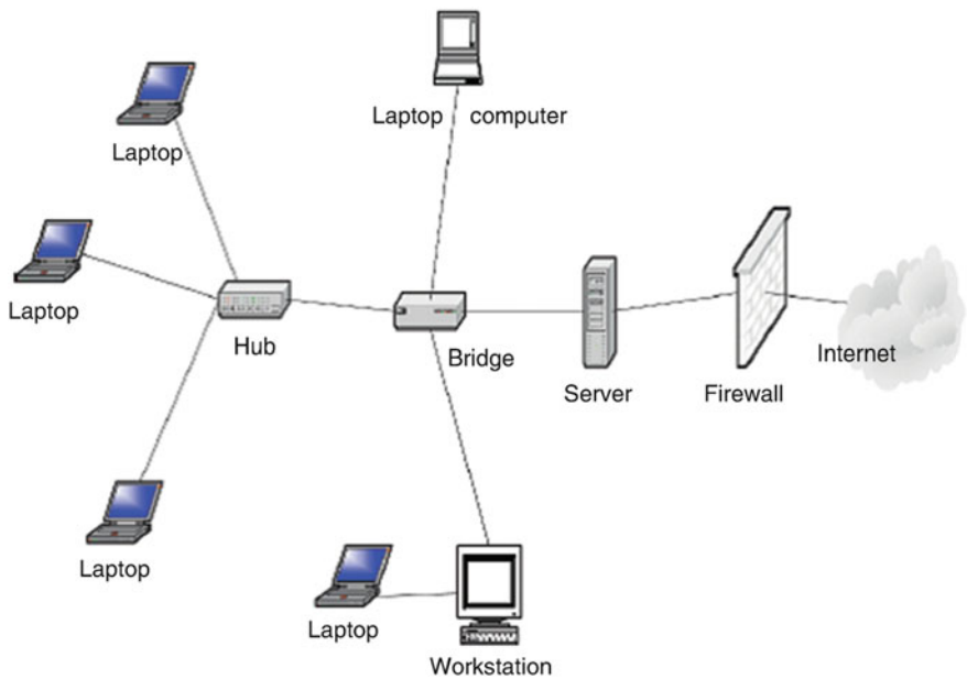
Fig. 1.27 Multiported bridge
