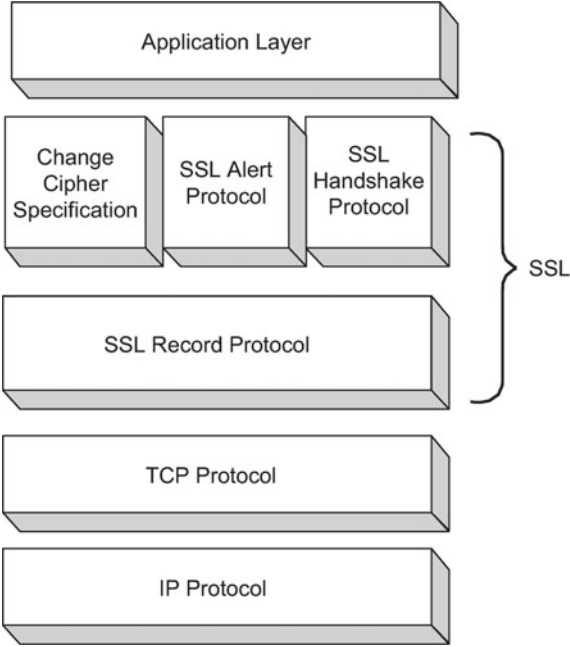
Fig. 18.5 SSL protocol stack
