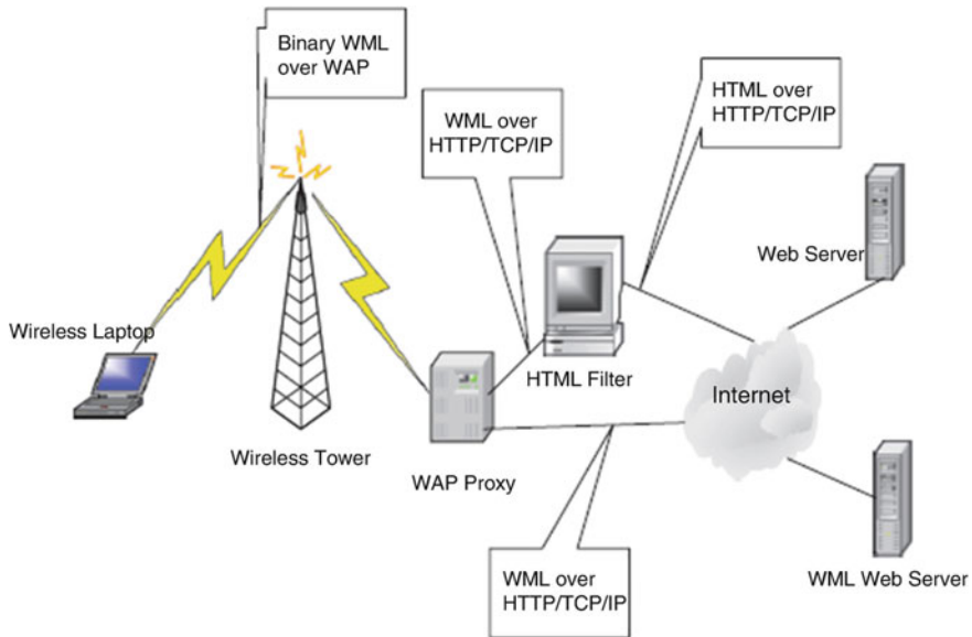
Fig. 19.9 WAP architecture infrastructure
