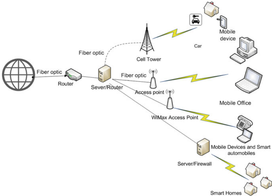
Fig. 19.1 Typical wireless broadband network
