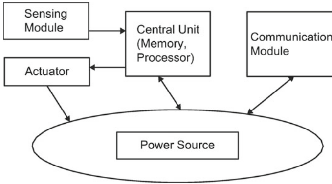
Fig. 20.1 Wireless sensor node
