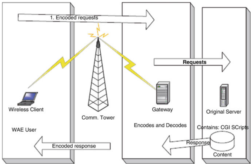
Fig. 19.8 WAP programming model
