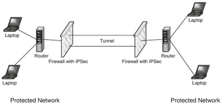
Fig. 18.13 Virtual private network (VPN) model
