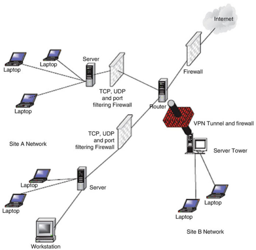
Fig. 12.3 TCP, UDP, and port number filtering firewall
