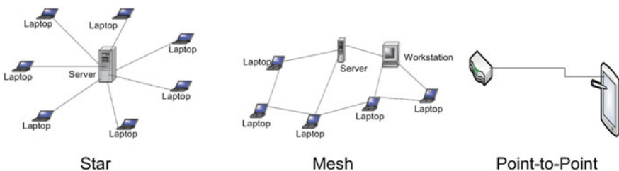
Fig. 25.2 Current IoT topologies
