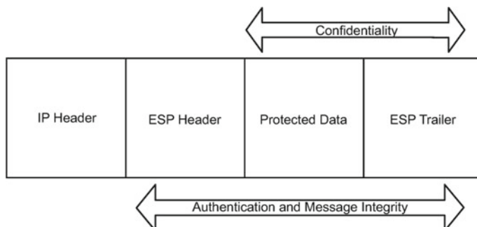
Fig. 18.9 IPsec's ESP protocol protection
