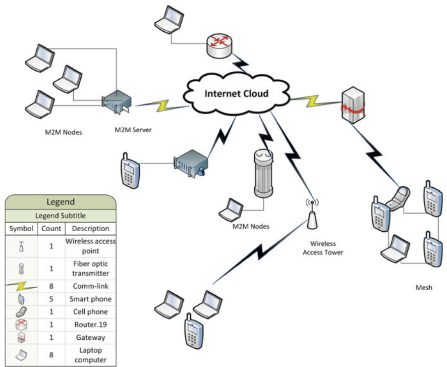
Fig. 25.3 IoT communication network architecture
