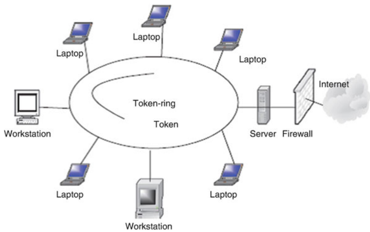
Fig.1.16 Token ring hub
