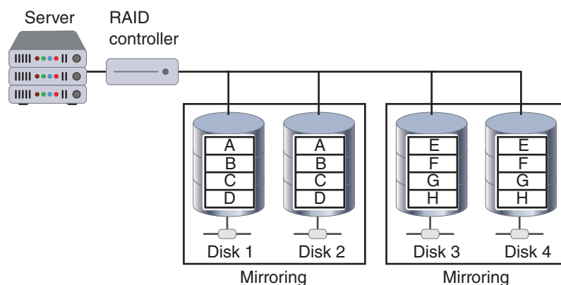
Figure 14-3 RAID Level 1
