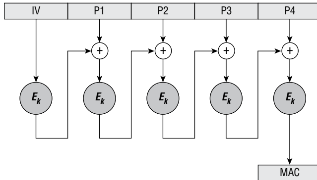
Figure 7.2: CBC-MAC example
