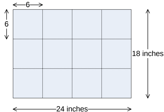
Figure 7.3: Cutting plywood
