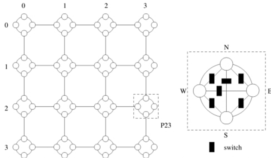
Figure 2.35. Switch connection patterns in a reconfigurable mesh.
