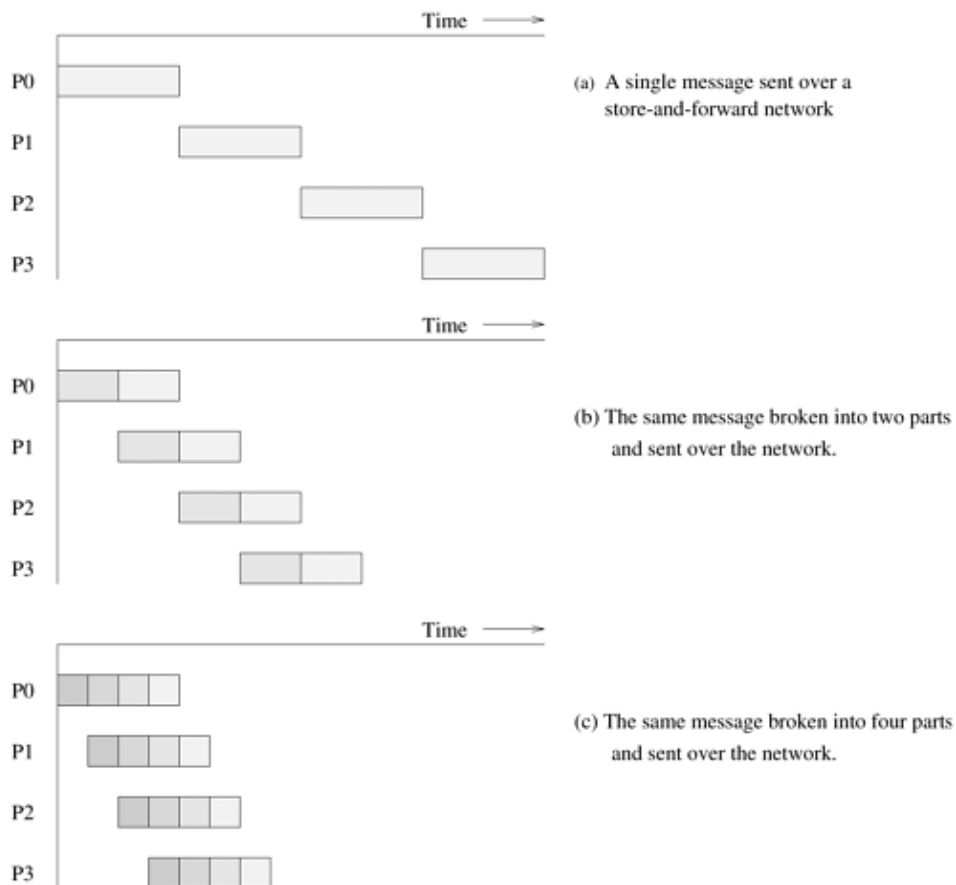
Figure 2.26. Passing a message from node P_0 to P_3 (a) through a store-and-forward communication network; (b) and (c) extending the concept to cut-through routing. The shaded regions represent the time that the message is in transit. The startup time associated with this message transfer is assumed to be zero.
