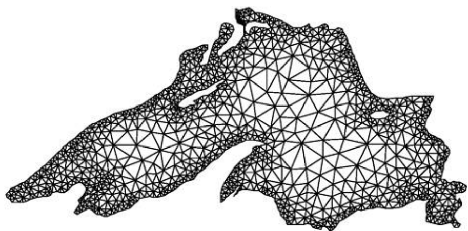
Figure 3.34. A mesh used to model Lake Superior.
