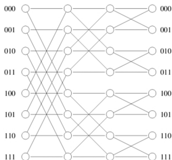
Figure 2.34. A Butterfly network with eight processing nodes.
