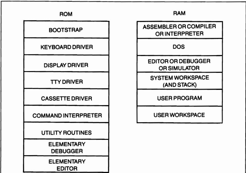
Figure 9.3: A memory map for a typical development system, showing the available software packages.
