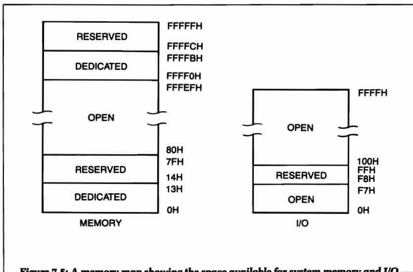
Figure 7.5: A memory map showing the space available for system memory and I/O.
