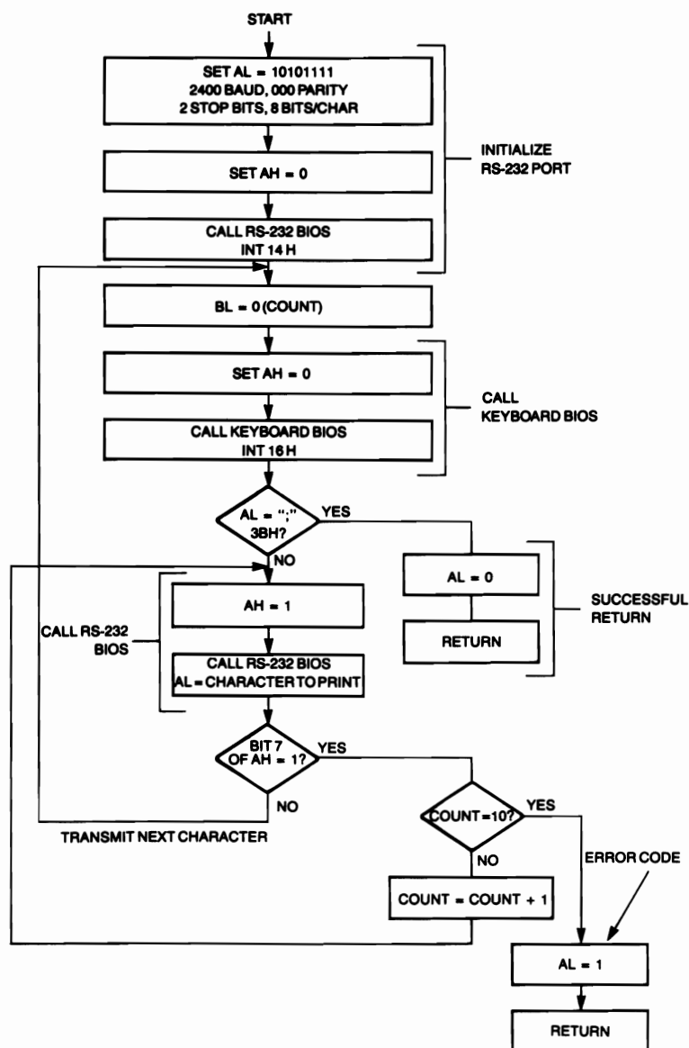
Figure 8.8: A flowchart for reading a character from the keyboard and then sending the character over the RS-232 communication line.
