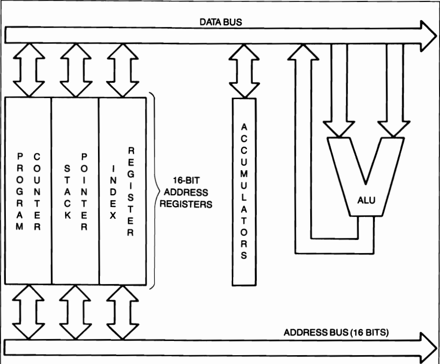
Figure 2.4: The PC, SP, and index registers are common microprocessor registers used in forming a complete system address.
