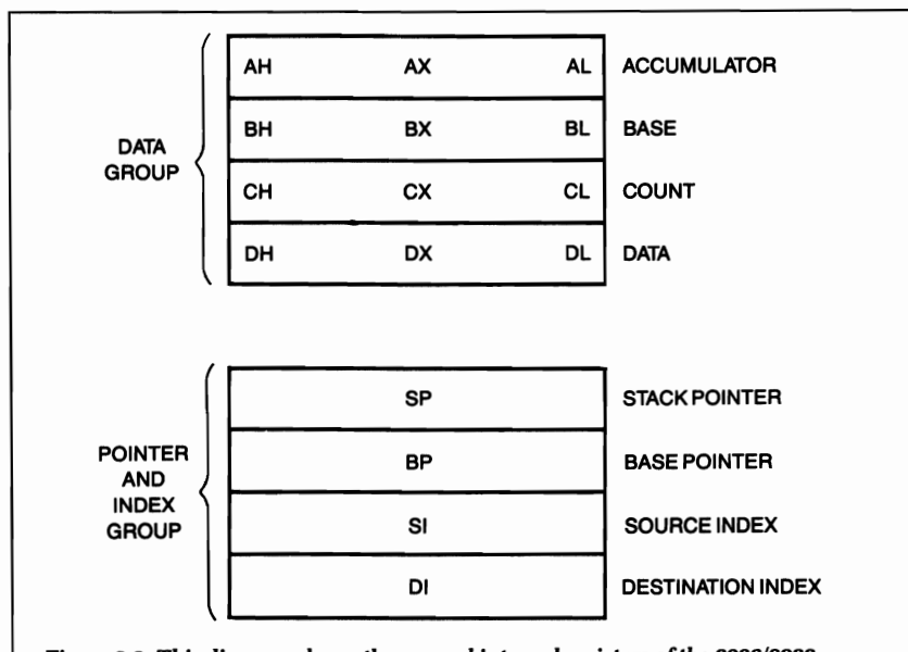
Figure 2.9: This diagram shows the general internal registers of the 8086/8088.
