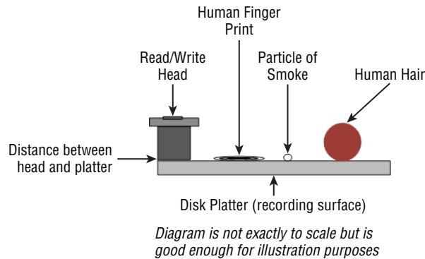
FIGURE 2.3 Head flying height
