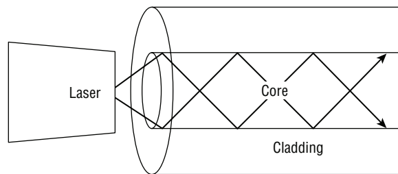
FIGURE 5.6 Multi-mode fiber carrying two beams of light
