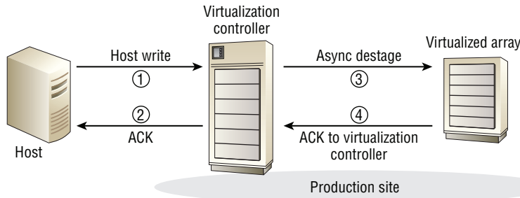
FIGURE 9.10 Write I/O to a virtualized storage array
