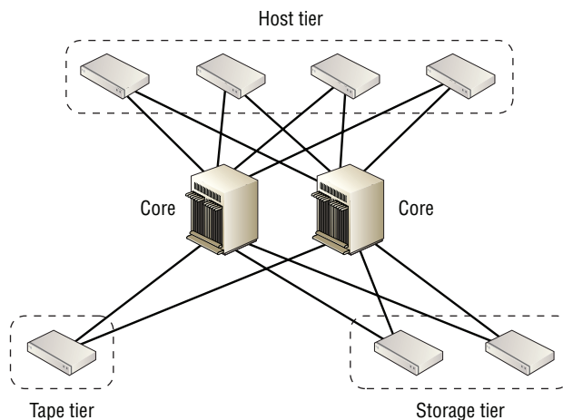
FIGURE 5.20 Tiered fabric topology
