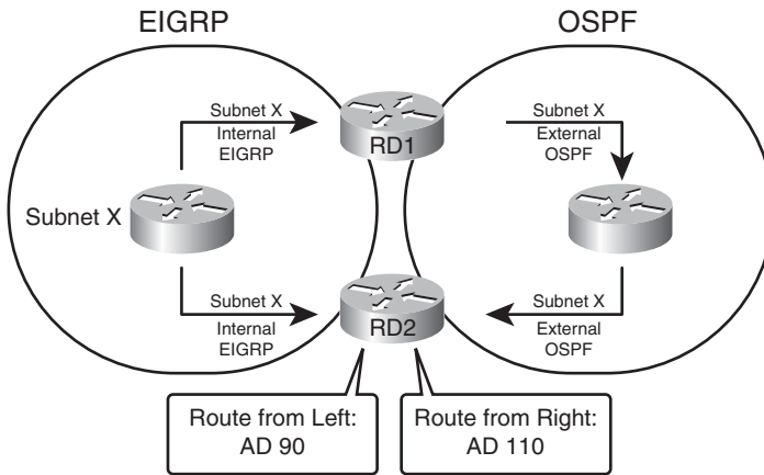
Figure 10-4 Subnet X: Internal EIGRP, External OSPF, on Router RD2
