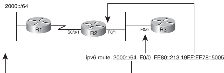
Figure 17-4 Static IPv6 Route on Router R3
