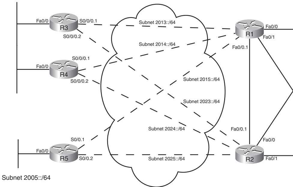
Figure 17-1 Sample Internetwork for IPv6 Routing Protocol Configuration
