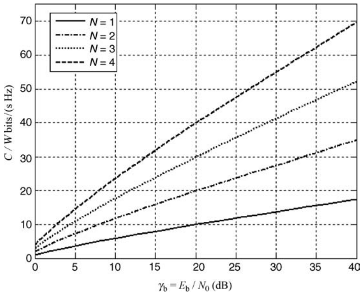
FIGURE 3.26 Comparison of the capacity of the SISO N \times N MIMO systems under ideal conditions.
