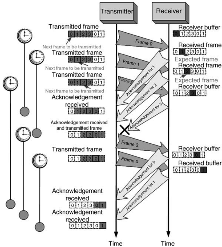
FIGURE 4.20 Go-back- N scheme in ARQ.
