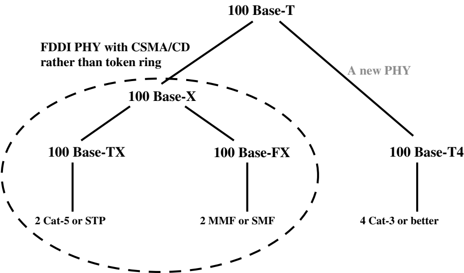
FIGURE 8.17 Overview of 100 Base-T fast Ethernet options.
