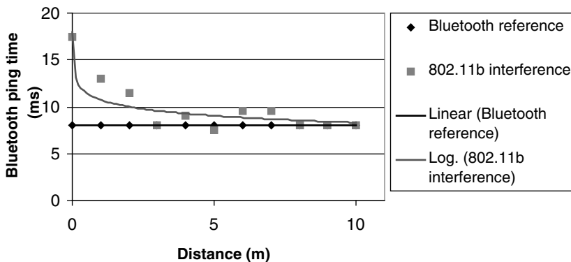
FIGURE 10.21 Bluetooth delay characteristics with and without 802.11b interference in an open office environment ad hoc network.
