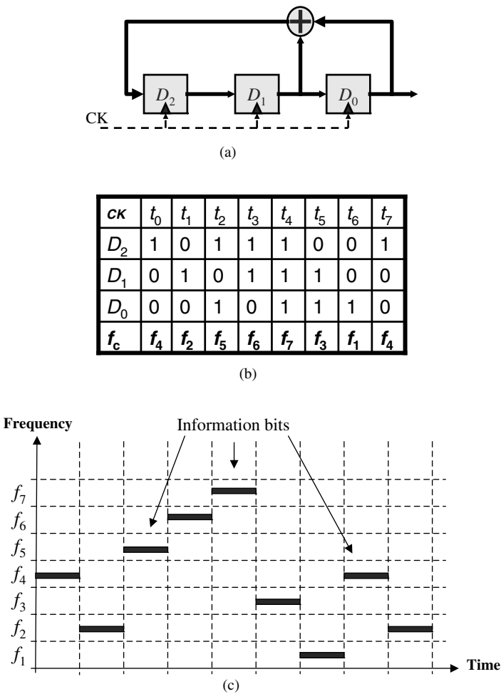
FIGURE 3.21 FHSS using a length-7 PN sequence: (a) three-stage state machine for implementation of the code; (b) states of the memory in time and frequency; (c) transmission of information bits in time and frequency in FHSS.
