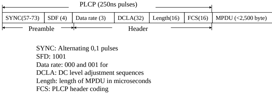
FIGURE 9.22 PLCP frame for the DFIR of the IEEE 802.11.
