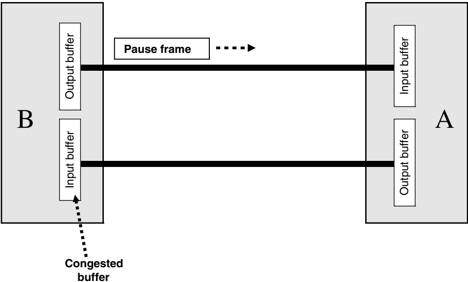
FIGURE 8.37 PAUSE frame application in full-duplex operation.
