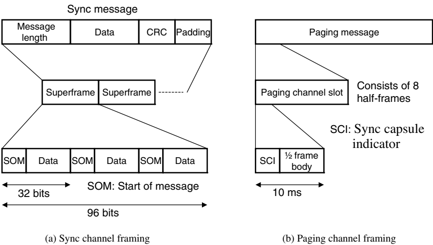
FIGURE 7.33 Framing in IS-95 forward channels.
