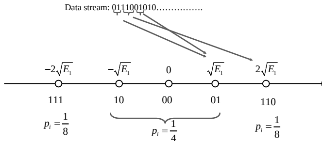
FIGURE 3.7 The signal constellation for 5-PAM.
