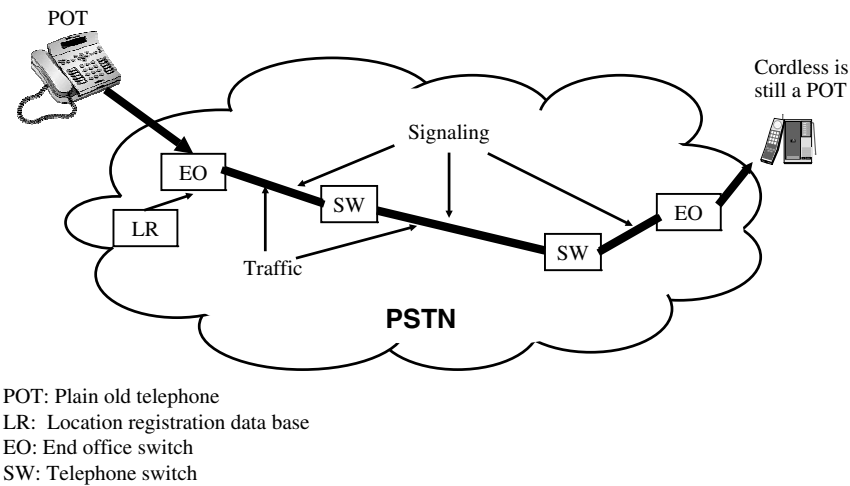
FIGURE 6.6 ISDN addressing connection-based PSTN.
