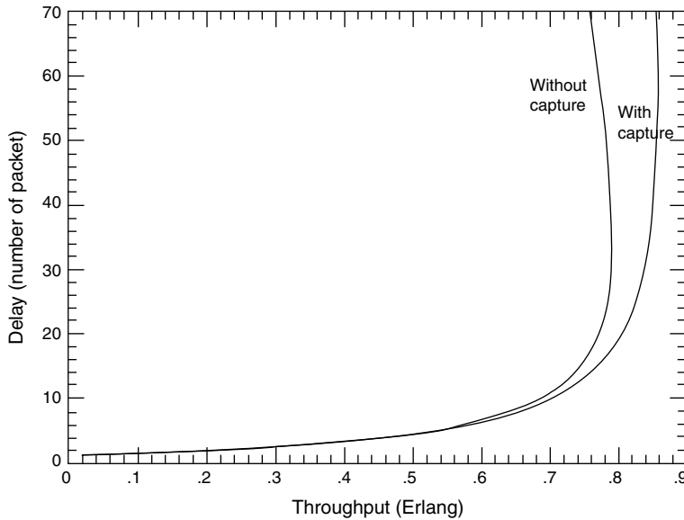
FIGURE 5.24 Delay versus throughput of CSMA for BPSK modulation and SNR of 20 dB, with and without capture.
