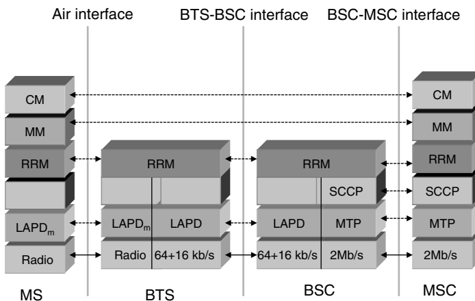
FIGURE 7.12 A typical protocol stack for a cellular network.
