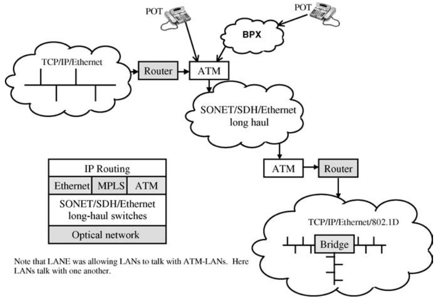
FIGURE 6.28 Integration of plain old telephone and LANs over long-haul optical fiber fabric.
