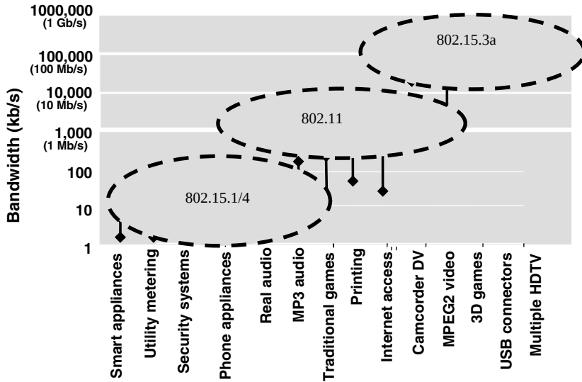
FIGURE 1.16 Applications bandwidth requirements and IEEE standards.
