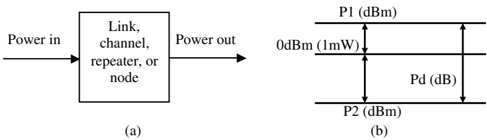
FIGURE A.1 Decibel: (a) Overall concept; (b) relation between dB and dBm.
