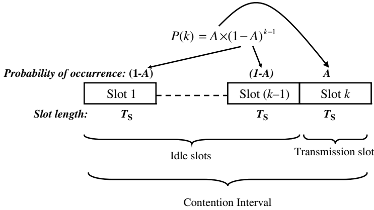
FIGURE 8.12 Contention interval and frame transmission.
