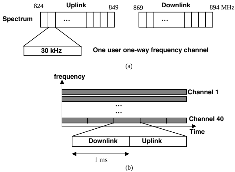
FIGURE 5.2 (a) FDMA/FDD in AMPS and (b) FDMA/TDD in CT-2.
