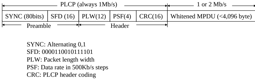
FIGURE 9.17 PLCP frame for the FH option in IEEE 802.11.
