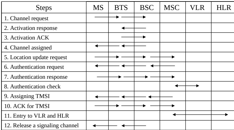
FIGURE 7.5 Registration procedure in a typical digital cellular network.
