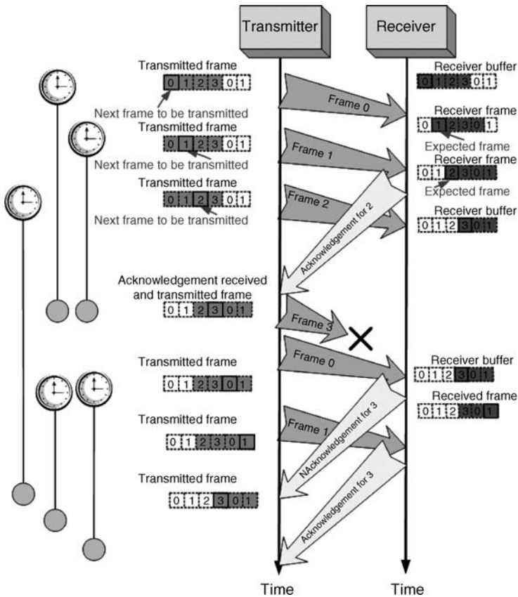
FIGURE 4.21 Selective repeat scheme in ARQ.
