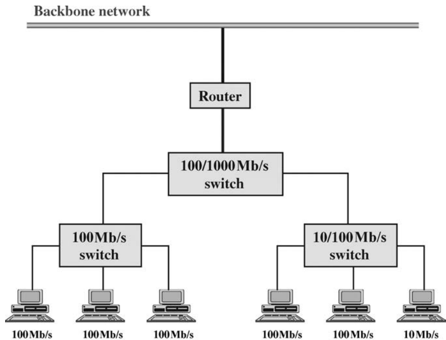
FIGURE 8.1 Hierarchical LANs.
