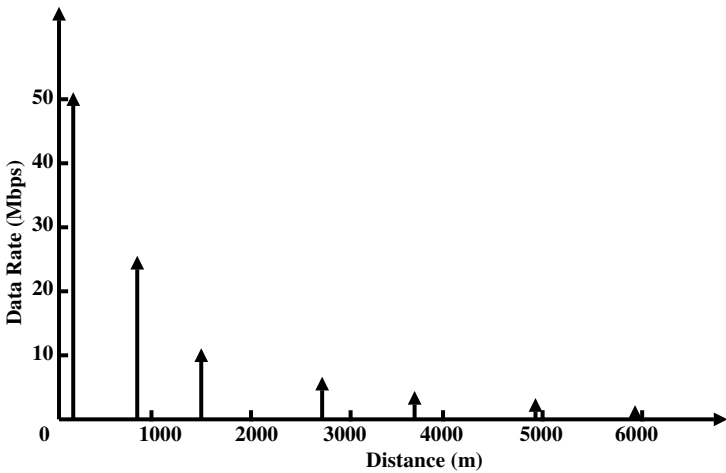
FIGURE P2.1 Data rate versus distance over a Cat-3 TP used for DSL modems.
