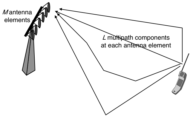
FIGURE 2.25 SIMO model.
