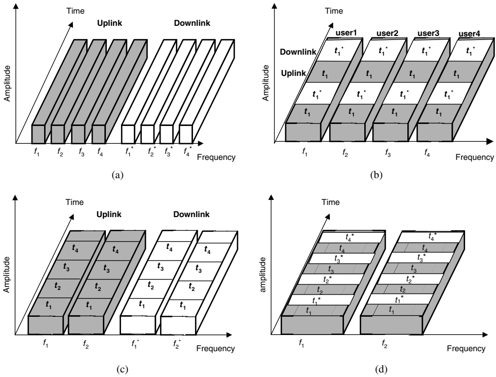
FIGURE 5.1 (a) FDMA/FDD; (b) FDMA/TDD; (c) TDMA/FDD with multiple carriers; (d) TDMA/TDD with multiple carriers.
