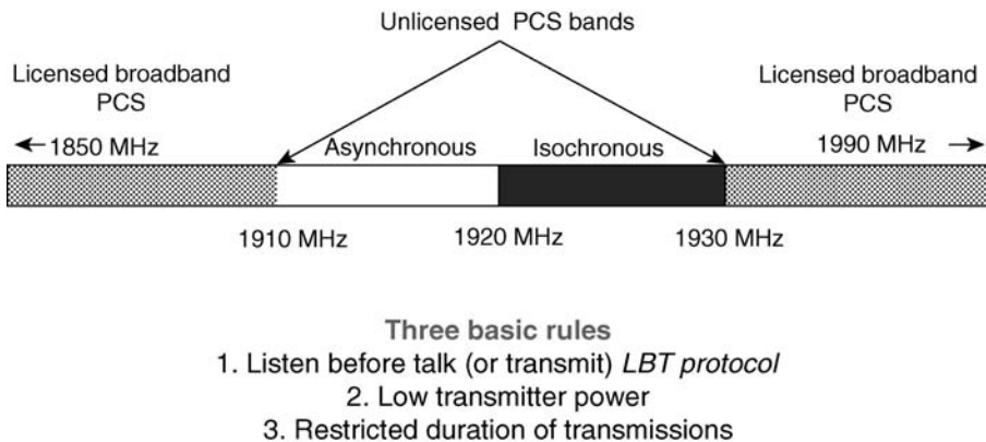
FIGURE 9.1 Unlicensed PCS bands and their spectrum etiquette.
