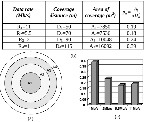
FIGURE 9.28 Data rates and coverage areas for the IEEE 802.11b in a semi-open indoor area: (a) coverage area for different data rates; (b) calculation of probabilities for data rates; (c) PDF of the data rates.
