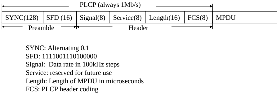
FIGURE 9.20 PLCP frame for the DSSS of the IEEE 802.11.
