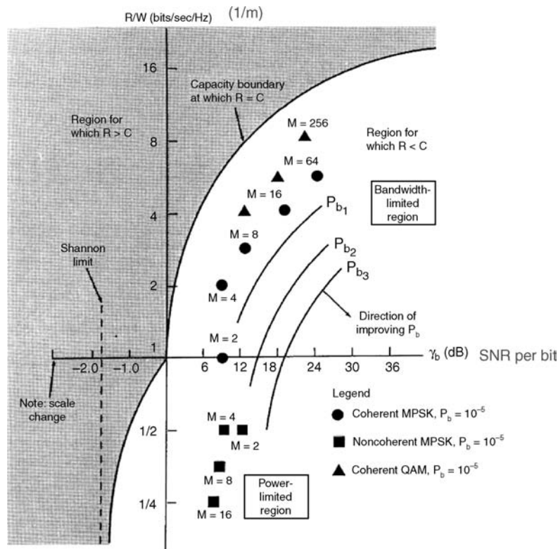
FIGURE 3.15 Channel capacity and comparison of several modulation methods at a BER of 10^{-5} . (Source: [Skl01] © Prentice Hall PTR.)
