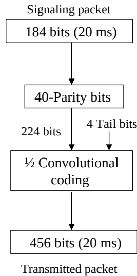
FIGURE 7.22 Coded signaling channel in GSM.
