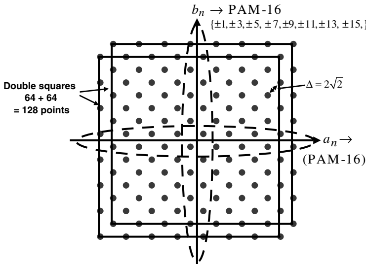
FIGURE 8.32 The double square 128-point (DSQ-128) constellation recommended by IEEE 802.3an for 10GBase-T.
