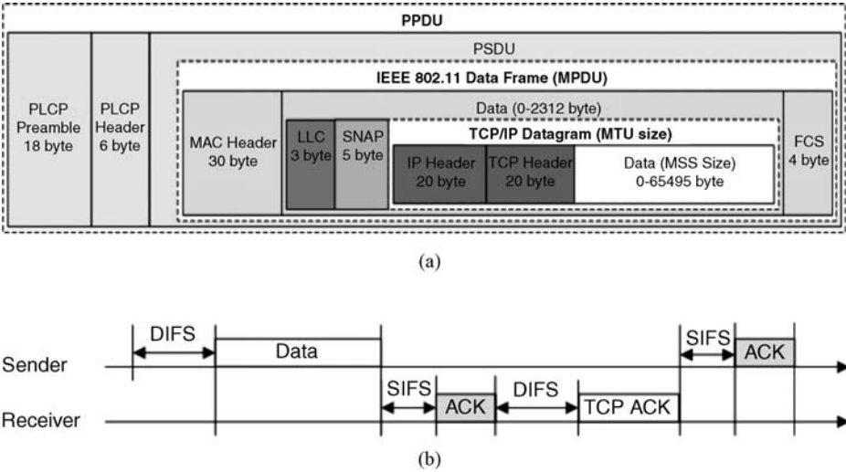
FIGURE P9.2 Packet transmission in the IEEE 802.11 b. (a) Overheads for the formation of a packet (b) overheads for successful transmission of a TCP packet.
