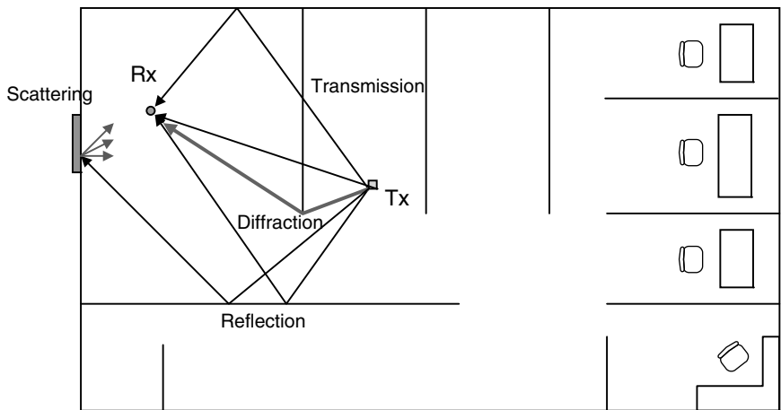
FIGURE 2.12 Radio propagation mechanisms in an indoor area.
