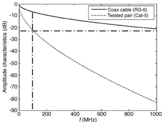
FIGURE 2.6 Amplitude characteristics of RG-6 coaxial cable and Cat-5 twisted-pair wiring for a cable with length of 100 m.
