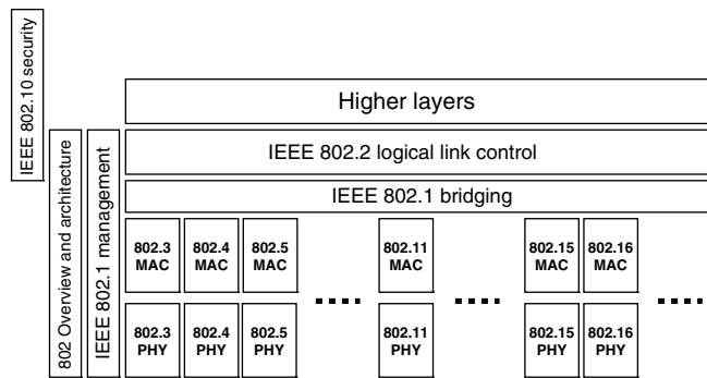
FIGURE 1.10 Organization of IEEE 802 standard series.
