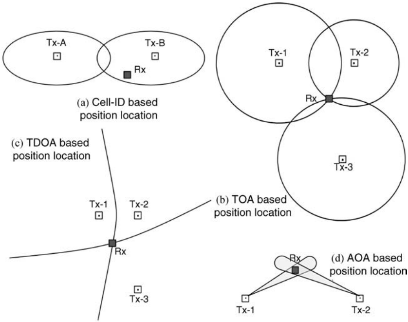
FIGURE 12.3 Location-sensing methodologies.
