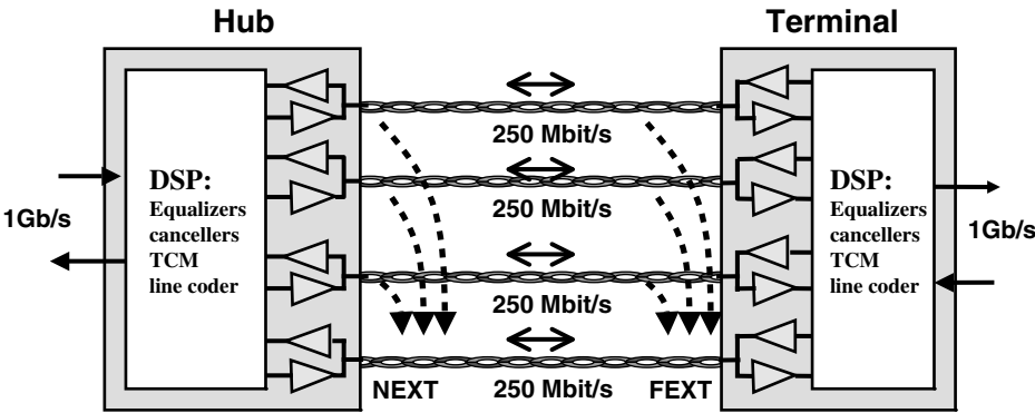
FIGURE 8.26 Overall operation of 1000Base-T.
