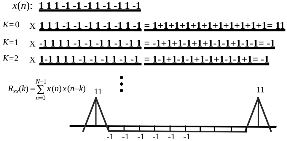
FIGURE 4.17 Autocorrelation of the Barker code.
