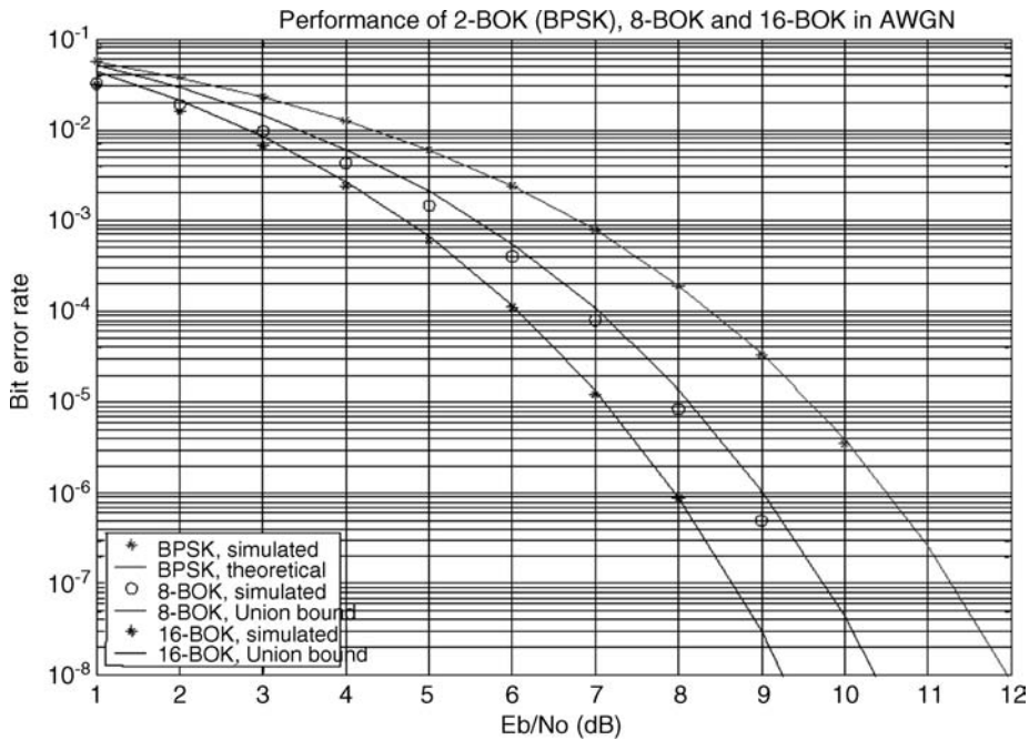
FIGURE 10.24 Theoretical and simulated performance of the M-BOK codes in AWGN [Wel03].
