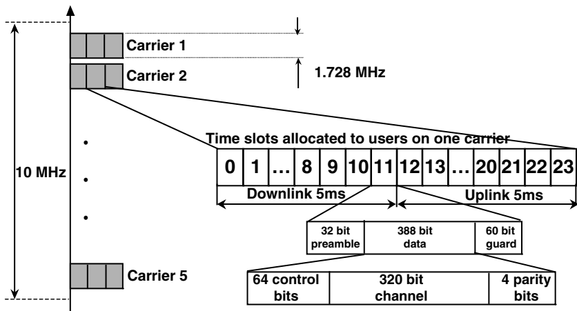
FIGURE 5.4 FDMA/TDMA/TDD in DECT.
