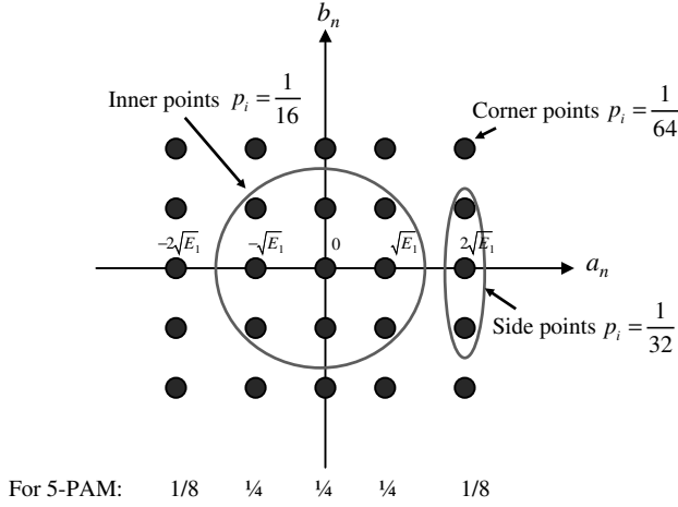
FIGURE 3.13 5 \times 5 PAM signal constellation used in different versions of Ethernet.
