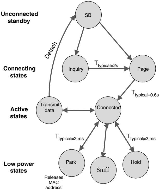
FIGURE 10.13 Functional overview of the Bluetooth specification.
