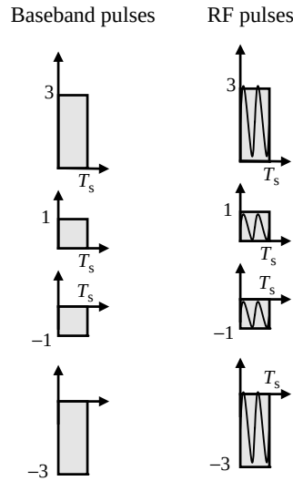
FIGURE 3.5 Baseband versus bandpass or RF transmission.
