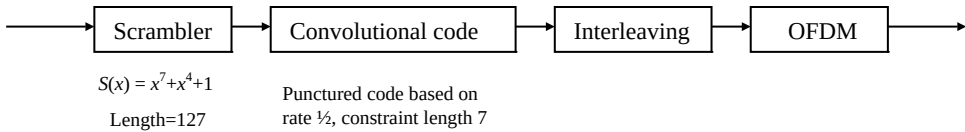
FIGURE 4.15 Overall block diagram of IEEE 802.11g using a scrambler to randomize data, convolutional codes for FEC, and block interleaving to spread blocks of errors.
