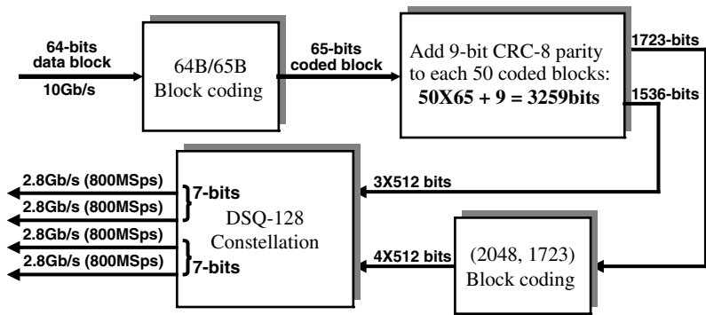
FIGURE 8.33 10GBase-T transmitter.
