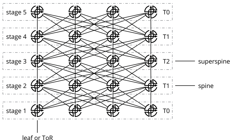
Figure 25-7 A five-stage spine and leaf
