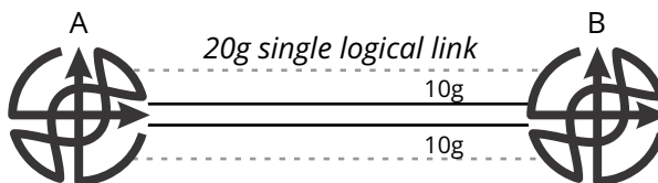
Figure 7-6 Link Aggregation
