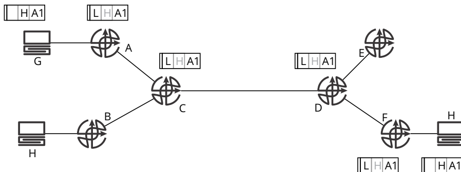
Figure 1-5 Label Switching
