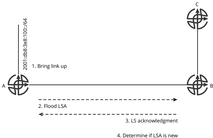
Figure 16-7 OSPF Flooding
