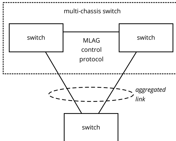
Figure 7-7 Multichassis Link Aggregation
