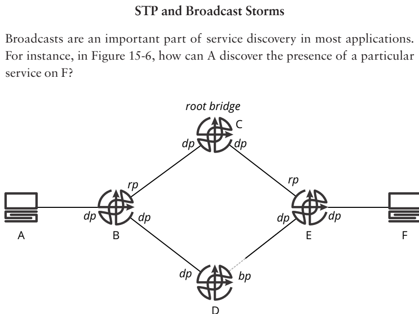
Figure 15-6 Broadcast Storms and the Spanning Tree Protocol
