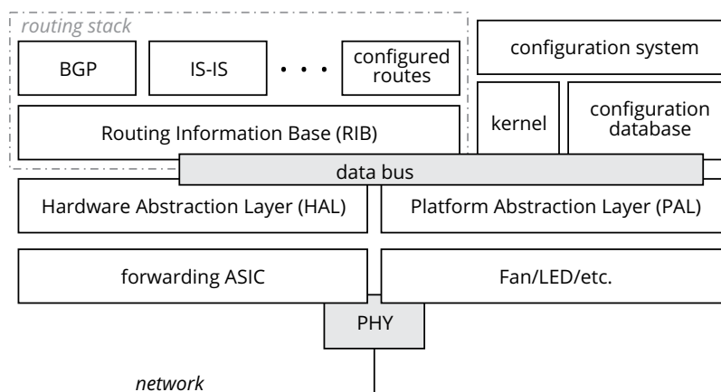
Figure 25-11 Router components
