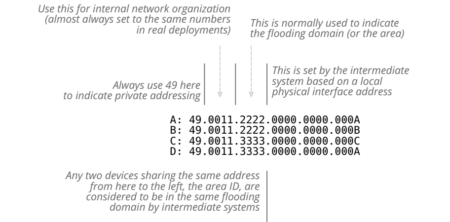
Figure 20-2 OSI addressing
