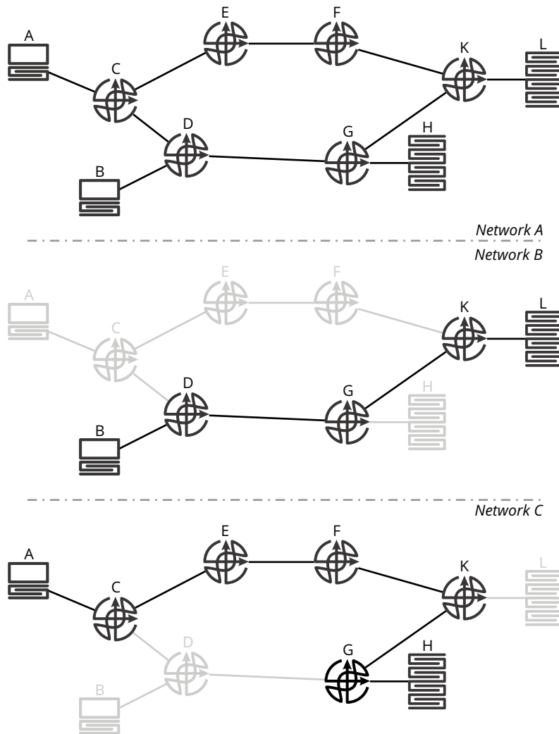
Figure 17-2 Overlays as a Form of Segmentation
