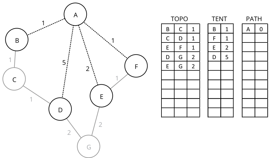
Figure 13-3 The Second Step in Dijkstra's SPF Calculation
