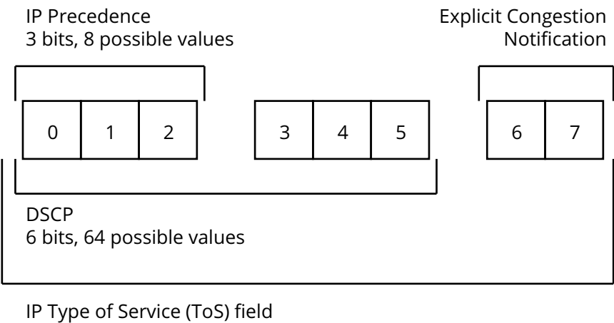
Figure 8-2 Ethernet DSCP and IP ToS Fields
