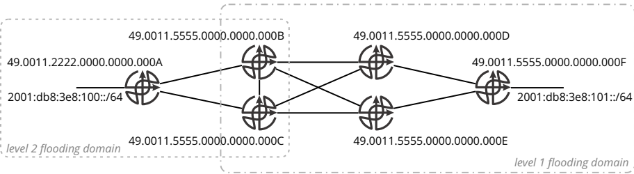
Figure 20-3 Flooding domains in IS-IS
