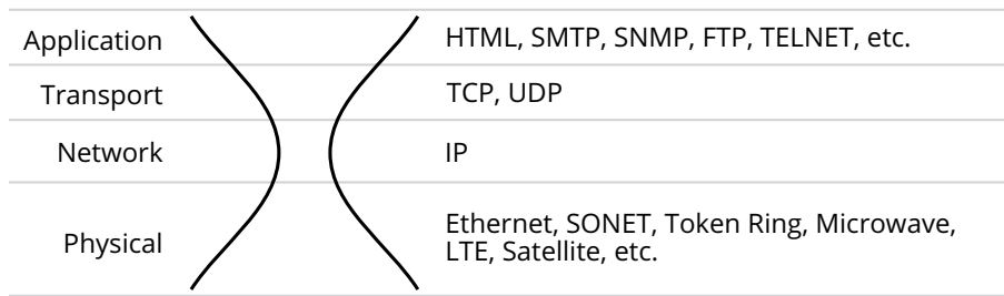
Figure 1-11 The DoD Model and the Wasp Waist
