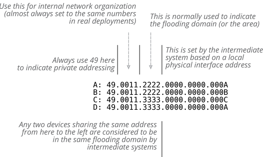
Figure 16-1 An Overview of the OSI Addressing Scheme Used in IS-IS
