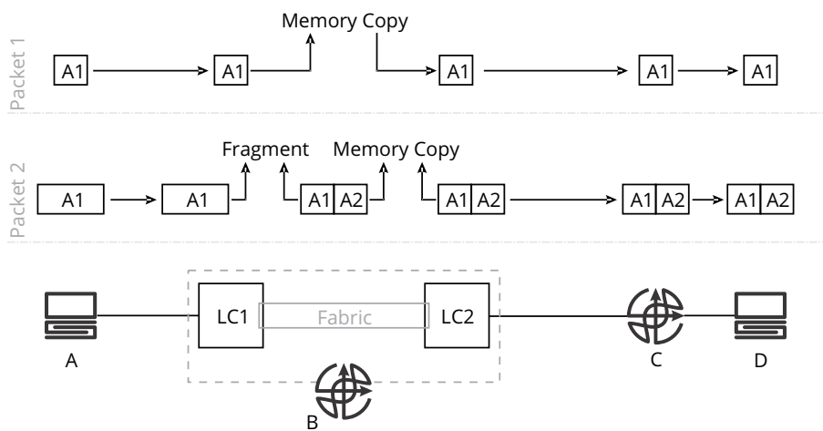
Figure 1-6 Fixed Cell Sizes
