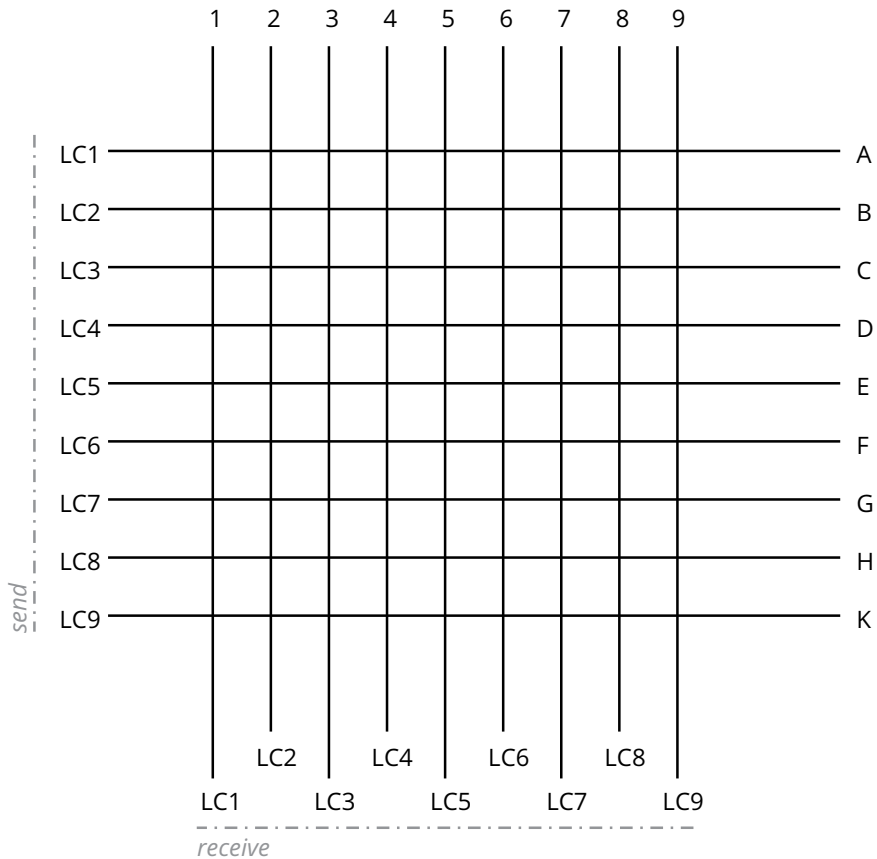
Figure 7-10 A Crossbar Fabric
