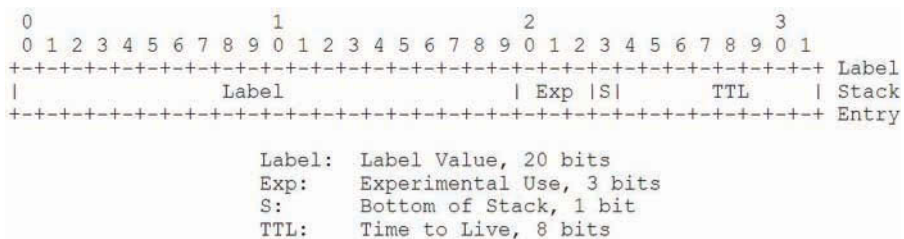
Figure 9-6 The MPLS Header
