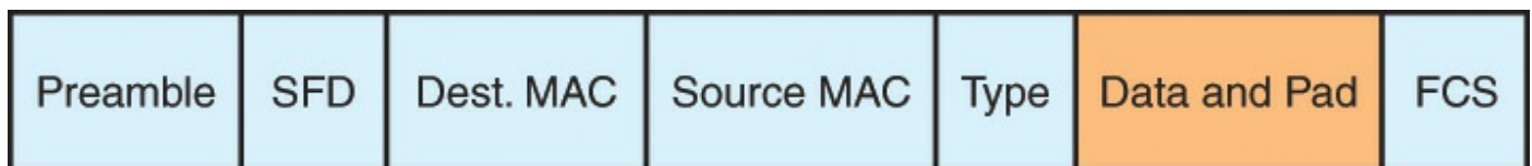
FIGURE 4.2 The Ethernet Frame Format
