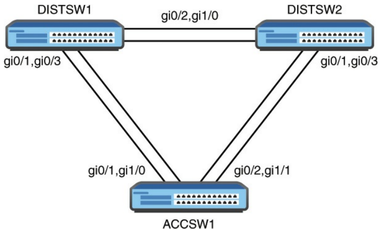
FIGURE 6.1 The EtherChannel Topology
