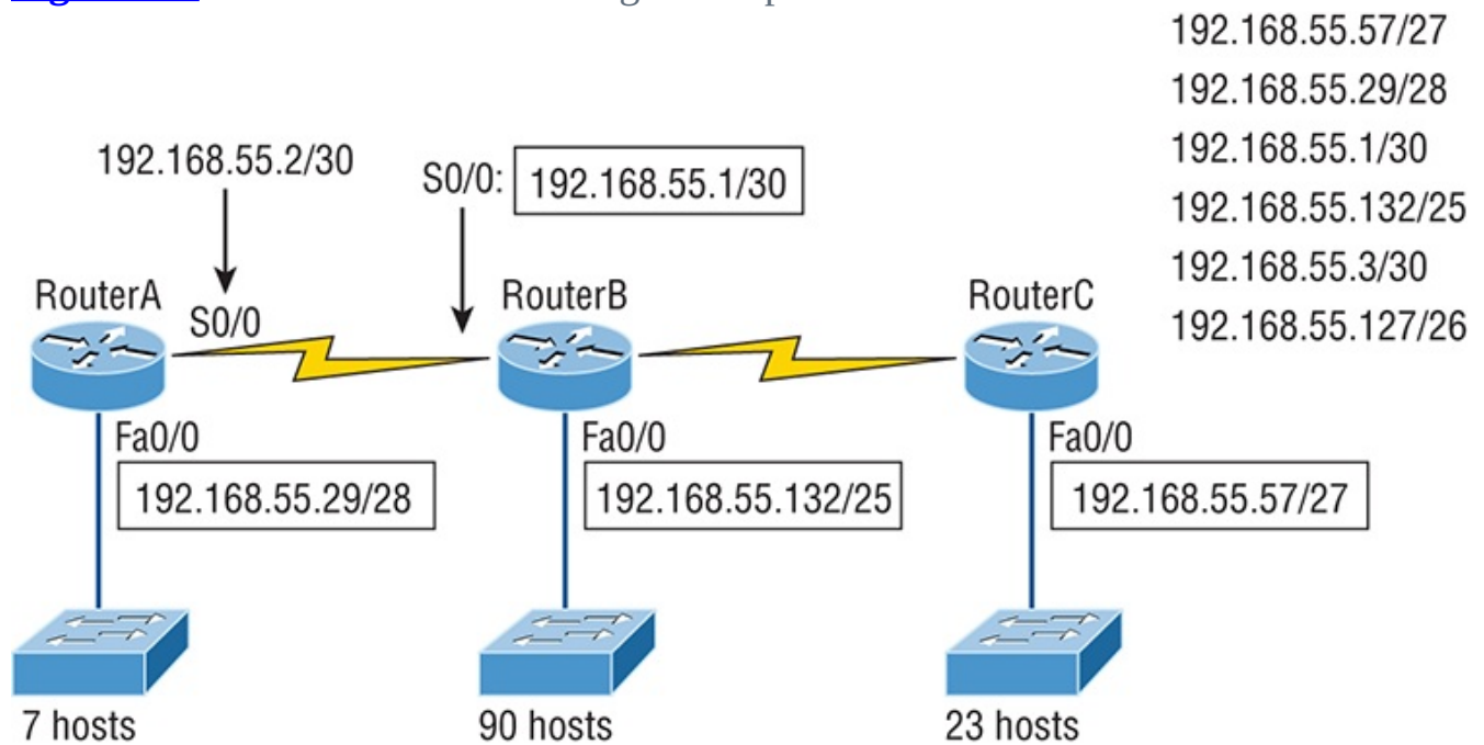
Figure 5-10: VLSM design example 2
