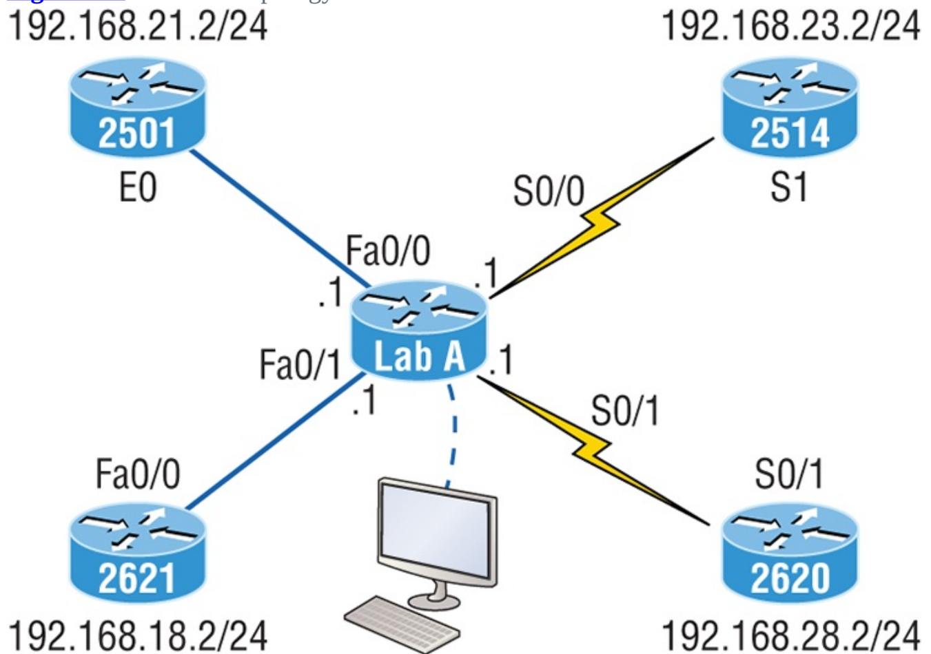
Figure 7-7: Network topology documented
