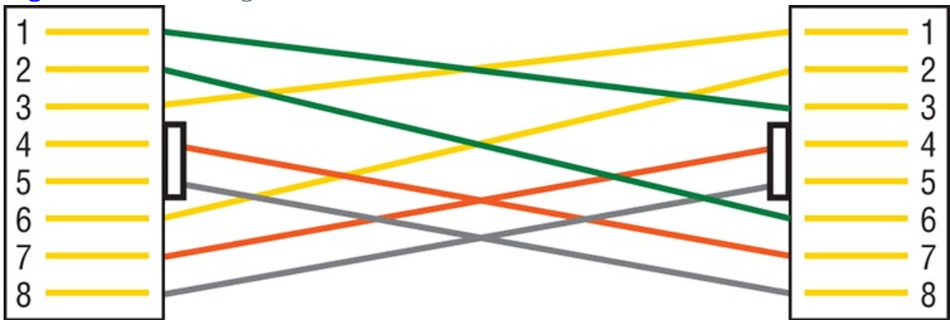
Figure 2-13: UTP Gigabit crossover Ethernet cable
