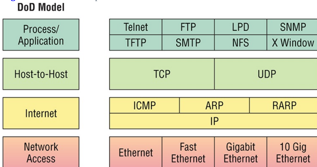
Figure 3-2: The TCP/IP protocol suite
