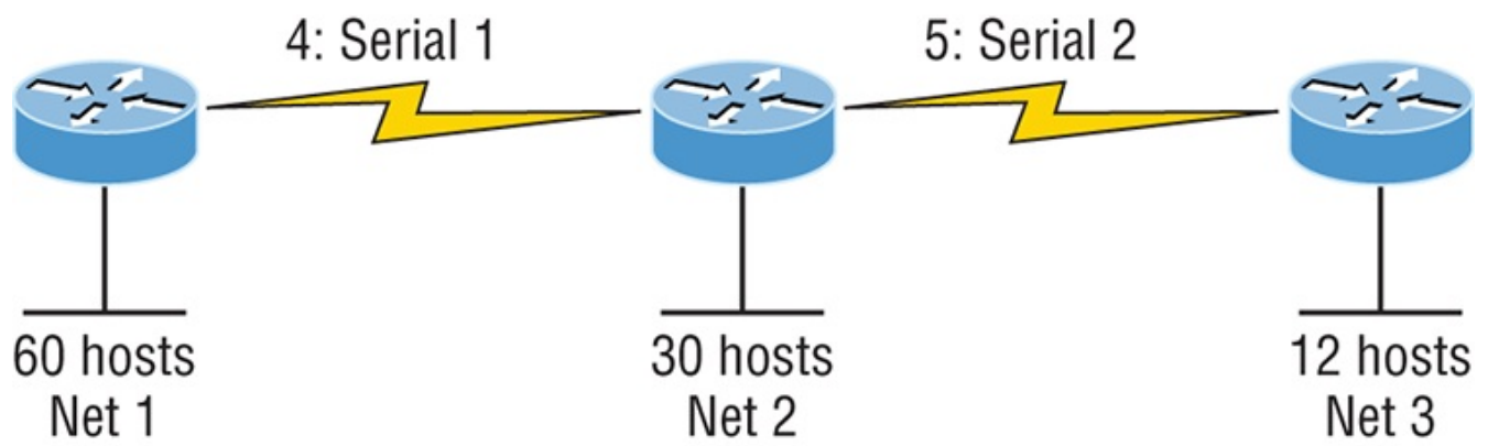
Figure 5-11: Solution to VLSM design example 2
