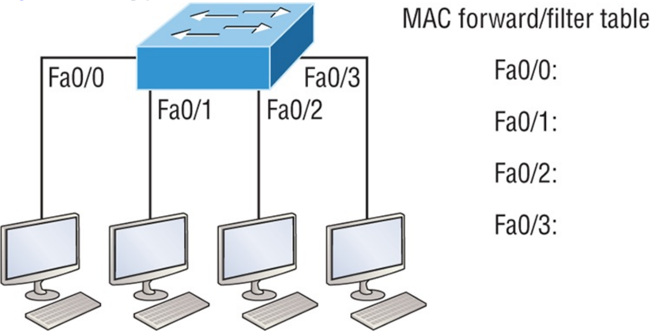
Figure 10-2: How switches learn hosts' locations
