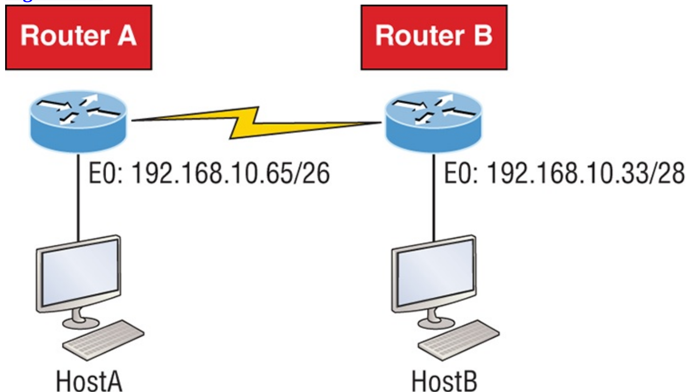
Figure 5-19: Find the valid host #2
