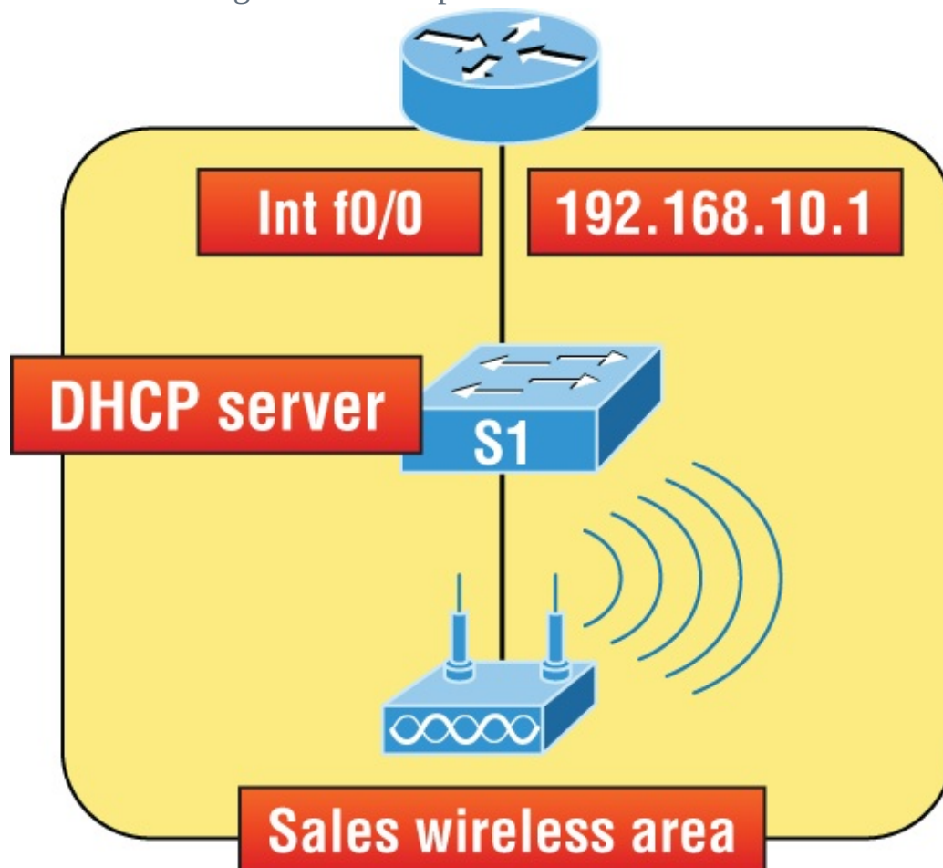
Figure 7-1: DHCP Configuration example on a switch
