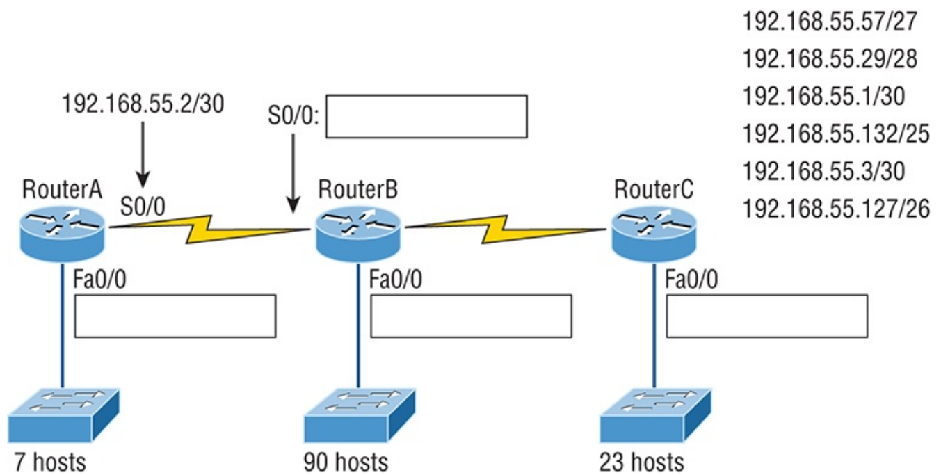
Figure 5-9: Solution to VLSM design example 1
