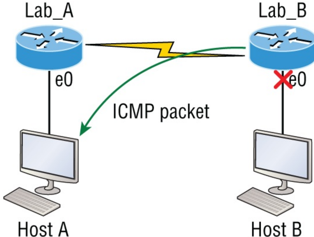
Figure 3-17: ICMP error message is sent to the sending host from the remote router.
