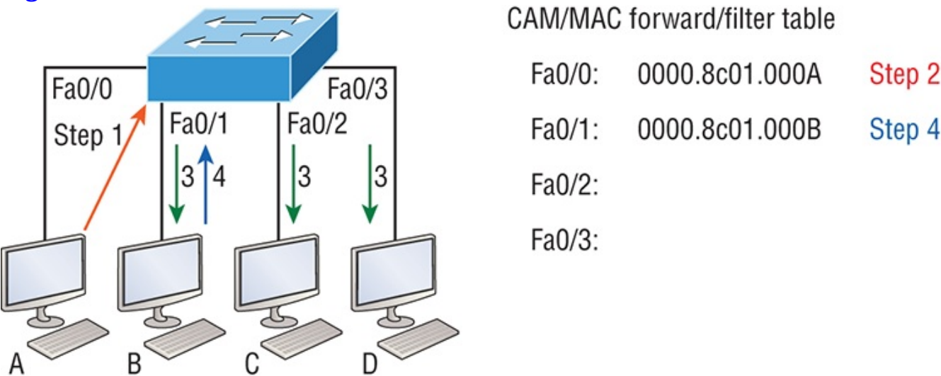
Figure 10-2: How switches learn hosts' locations
