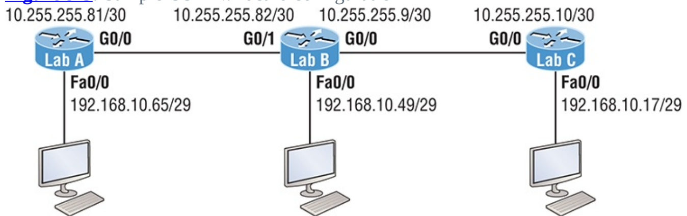
Figure 9-3: Sample OSPF wildcard configuration
