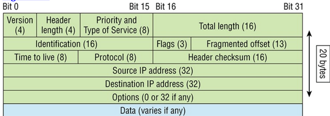
Figure 3-15: IP header
