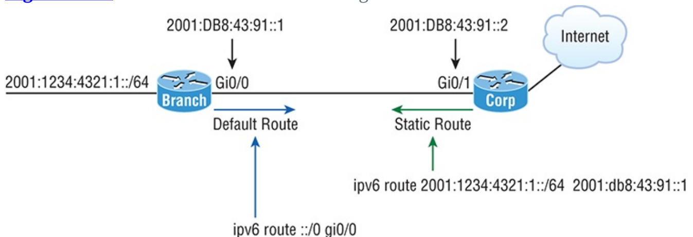
Figure 14-12: IPv6 static and default routing
