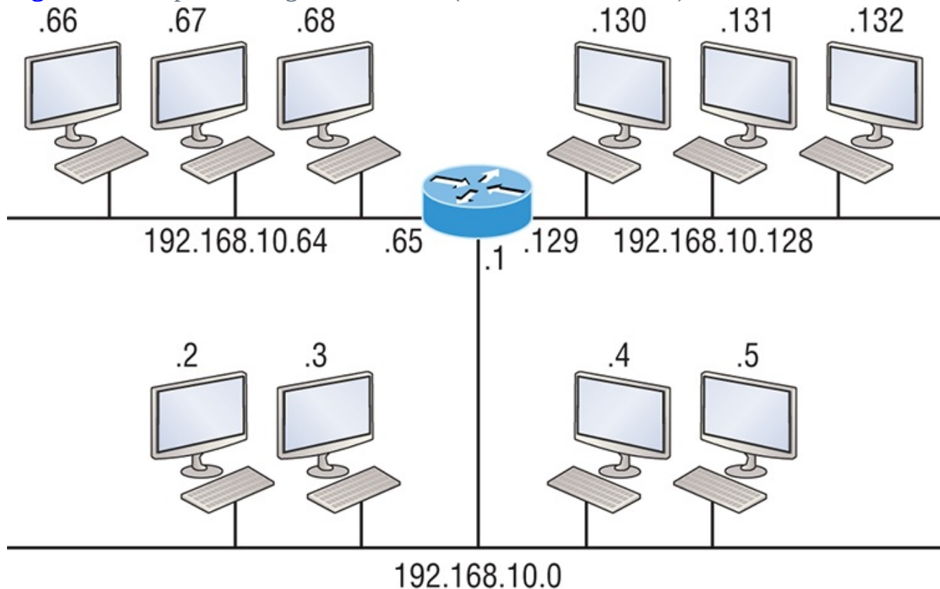
Figure 4-4: Implementing a class C /26 (with three networks)
