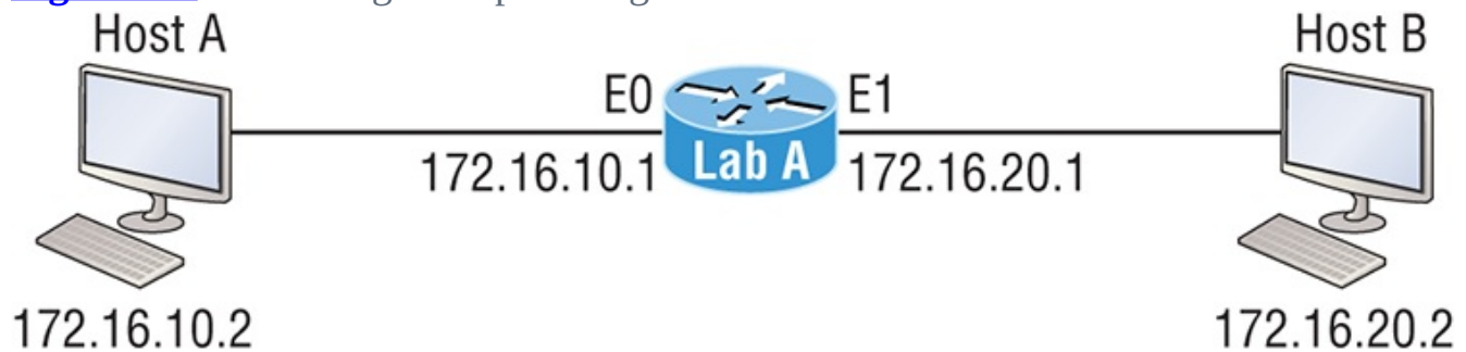
Figure 8-2: IP routing example using two hosts and one router
