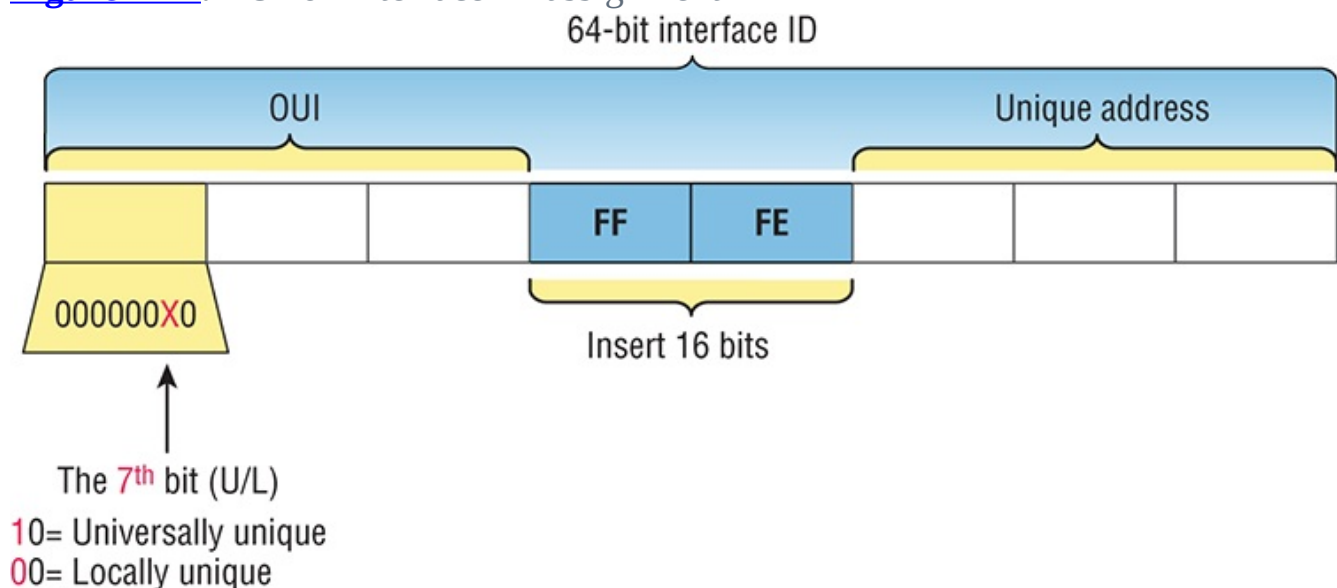
Figure 14-4: EUI-64 interface ID assignment
