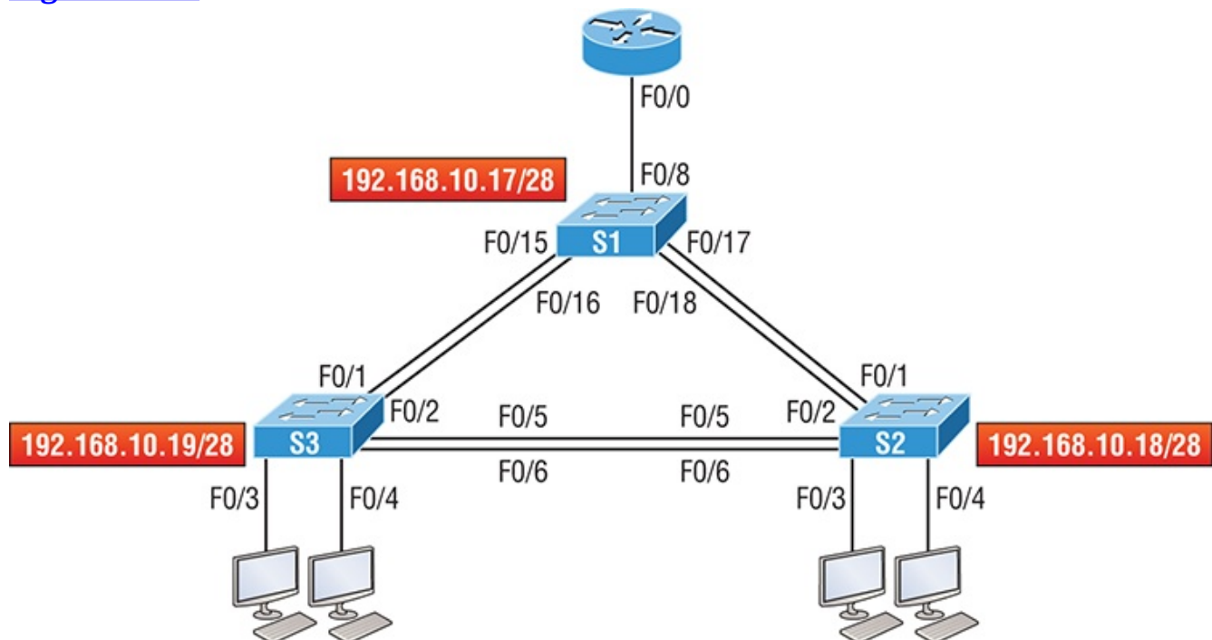
Figure 10-10: Our switched network
