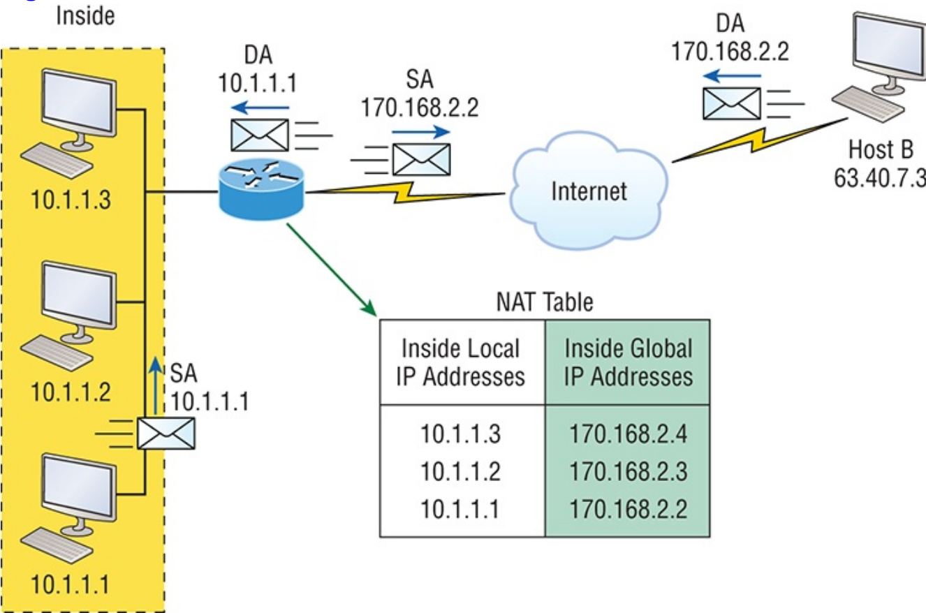
Figure 13-3: NAT overloading example (PAT)
