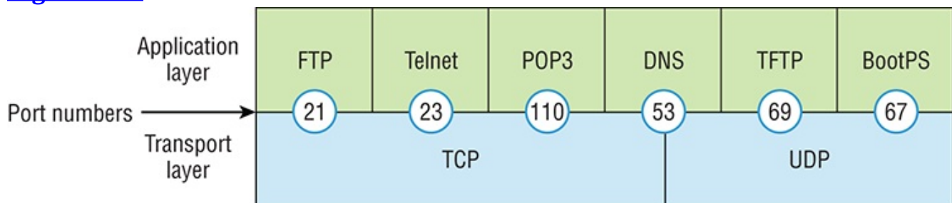
Figure 3-14: Port numbers for TCP and UDP
