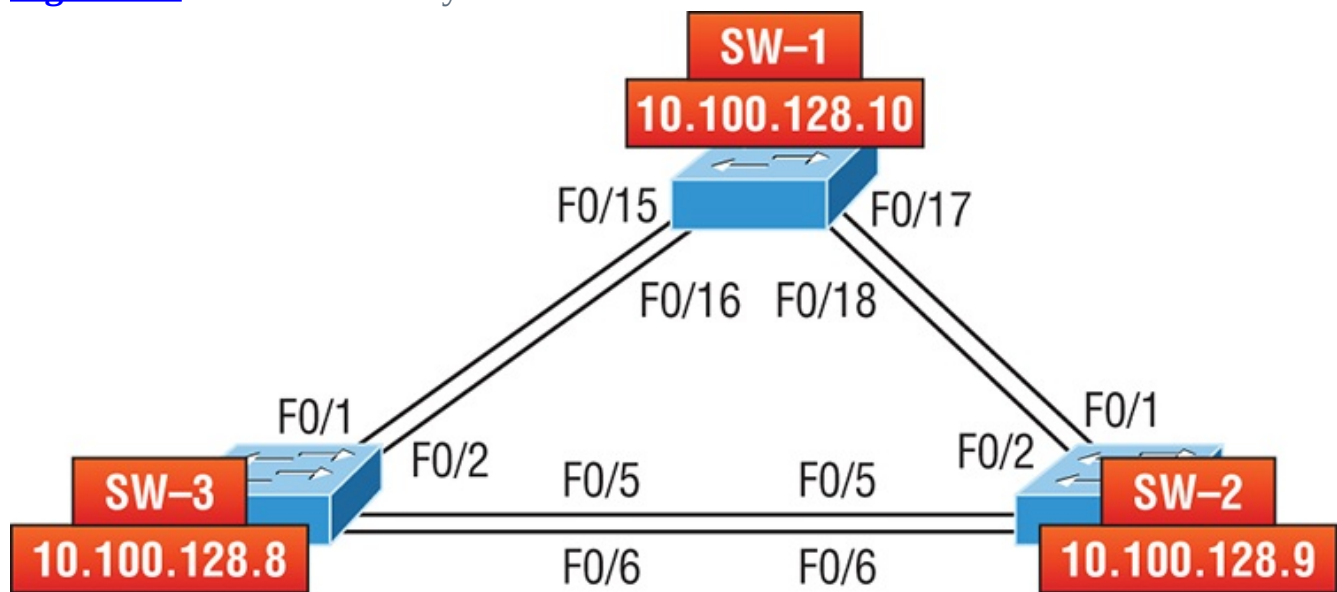
Figure 7-5: Cisco Discovery Protocol
