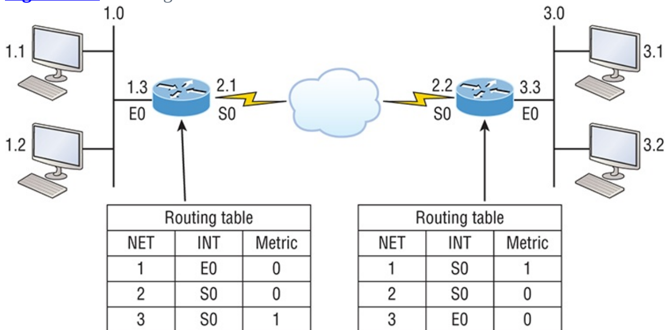
Figure 1-13: Routing table used in a router
