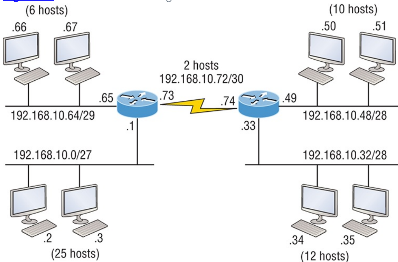
Figure 5-2: Classless network design
