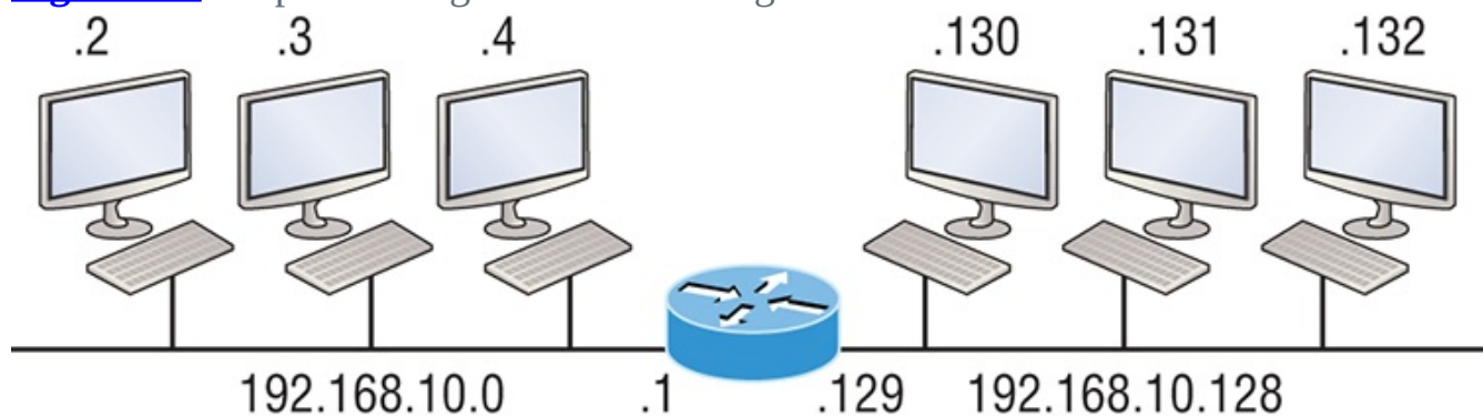
Figure 4-3: Implementing a Class C /25 logical network
