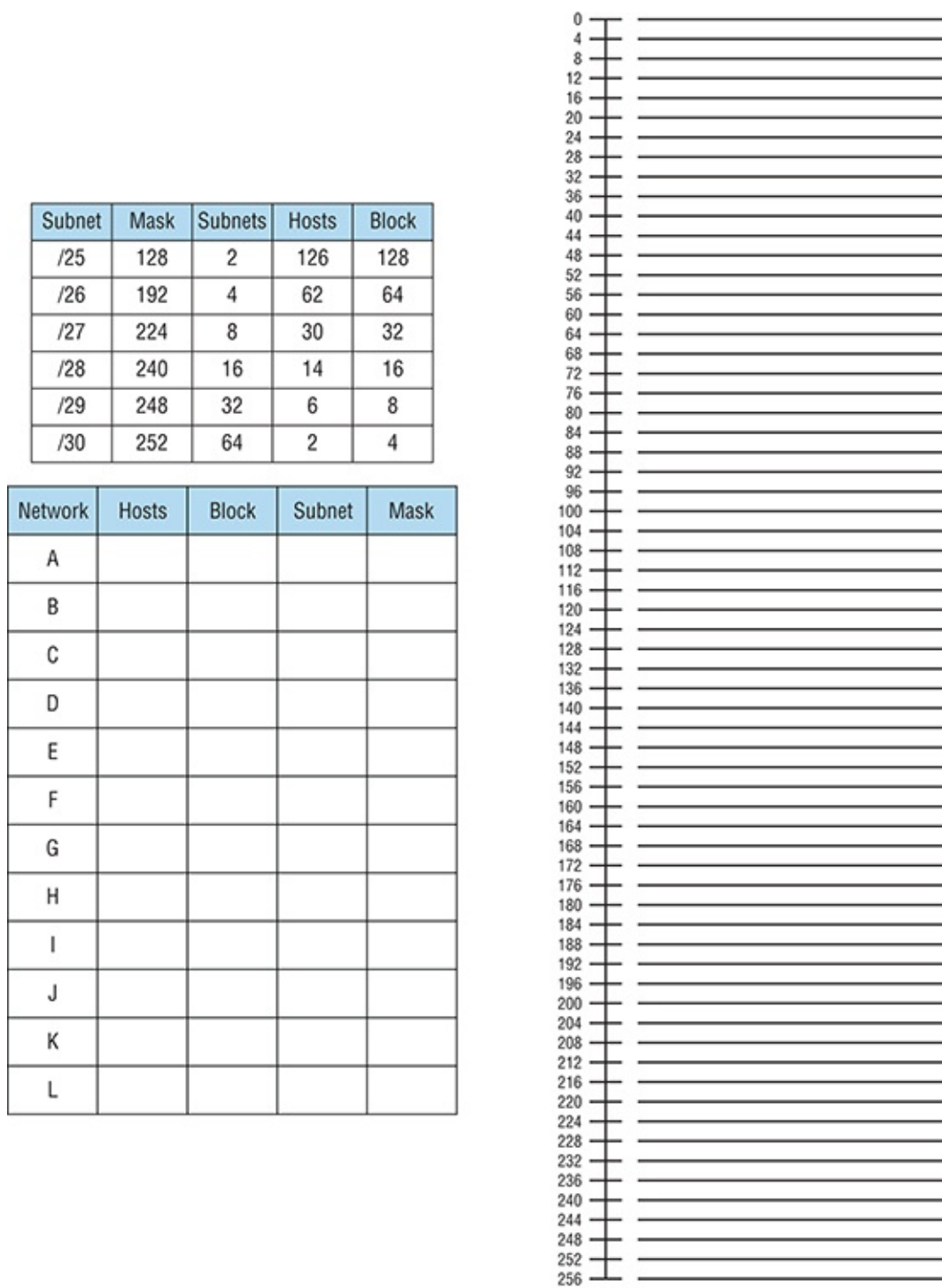
Figure 5-4: VLSM network example 1
