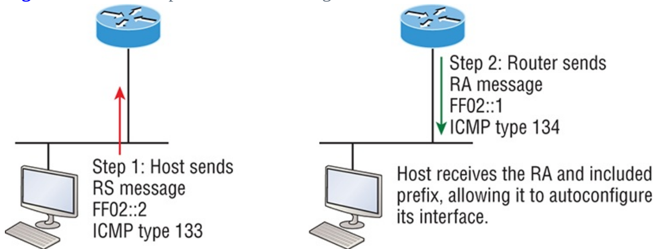
Figure 14-5: Two steps to IPv6 autoconfiguration
