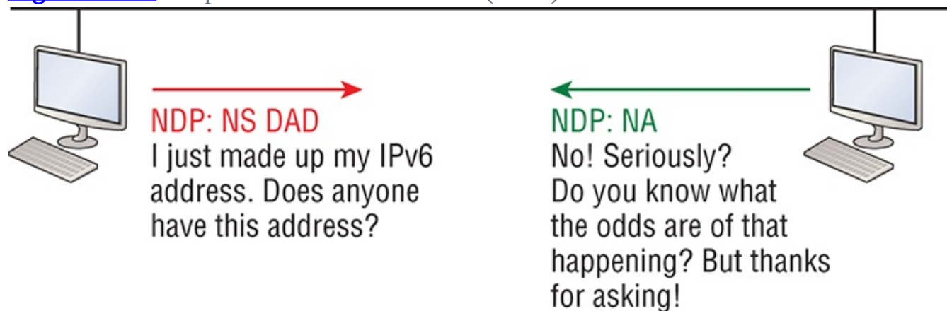
Figure 14-11: Duplicate address detection (DAD)
