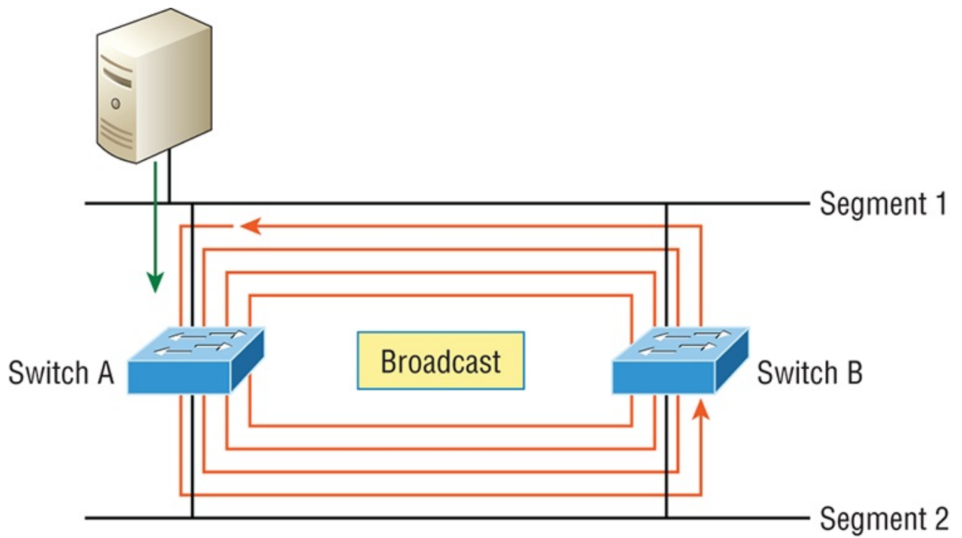
Figure 10-8: Multiple frame copies
