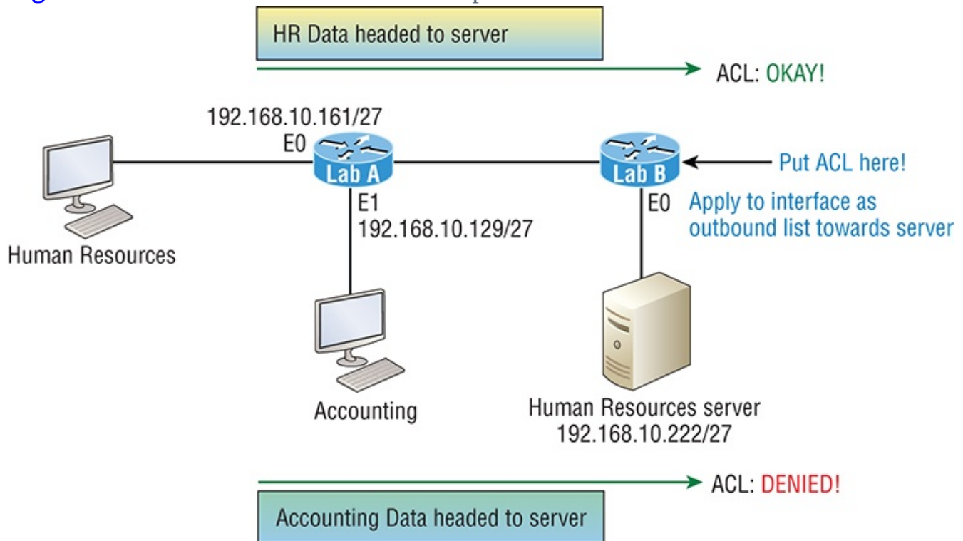
Figure 12-3: IP standard access list example 2
