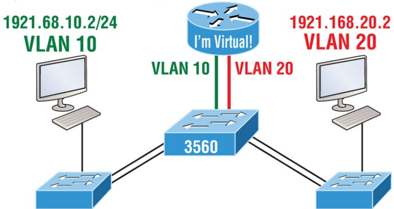
Figure 11-16: Inter-VLAN routing with a multilayer switch
