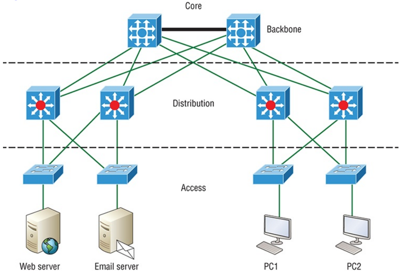
Figure 2-24: The Cisco hierarchical model
