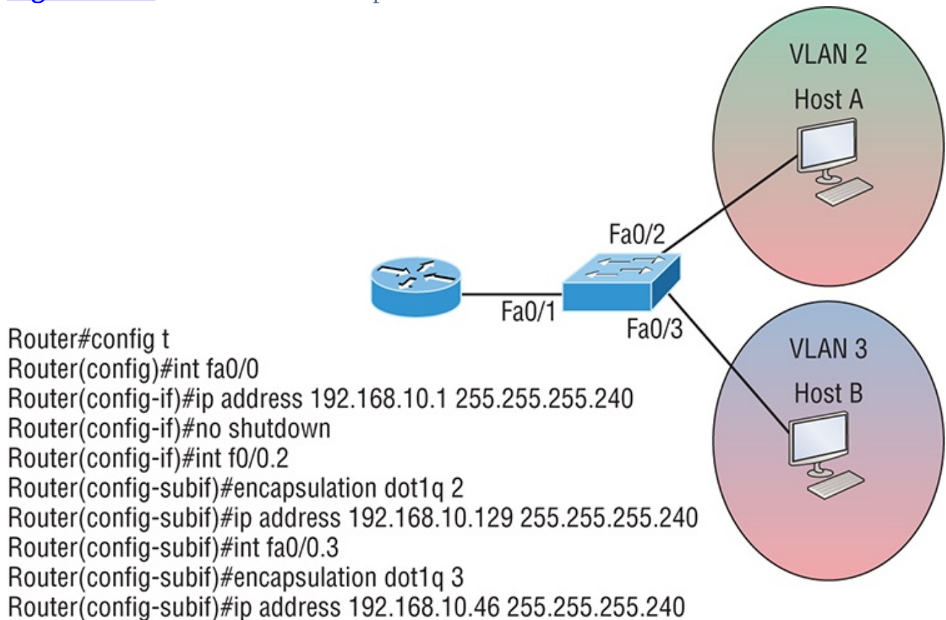
Figure 11-15: Inter-VLAN example 4
