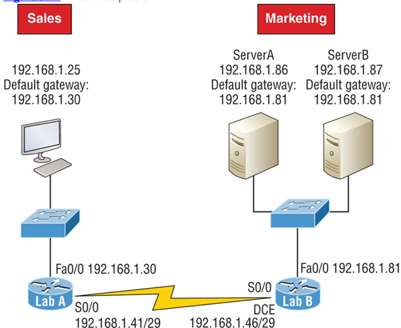
Figure 5-17: IP address problem 2
