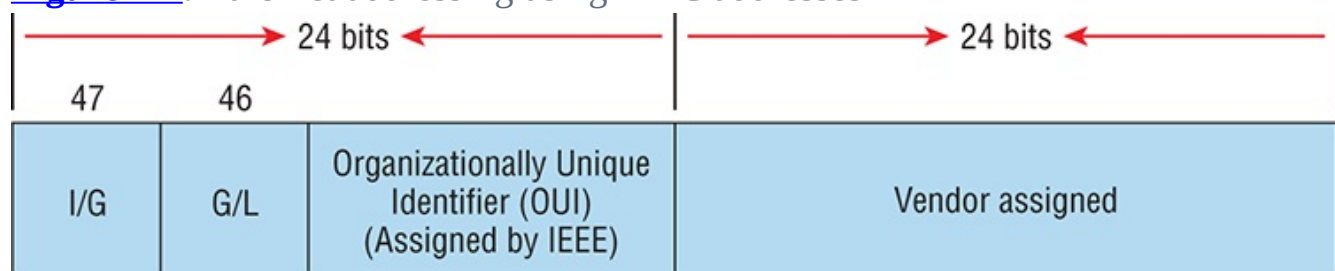
Figure 2-7: Ethernet addressing using MAC addresses
