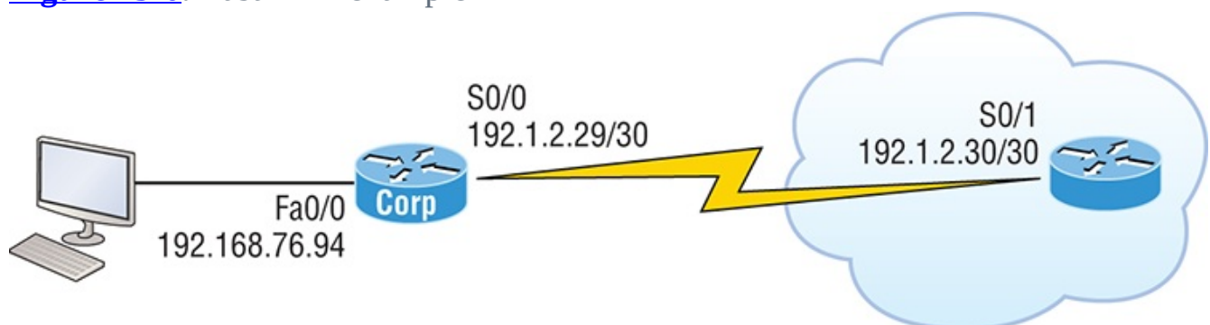
Figure 13-6: Last NAT example
