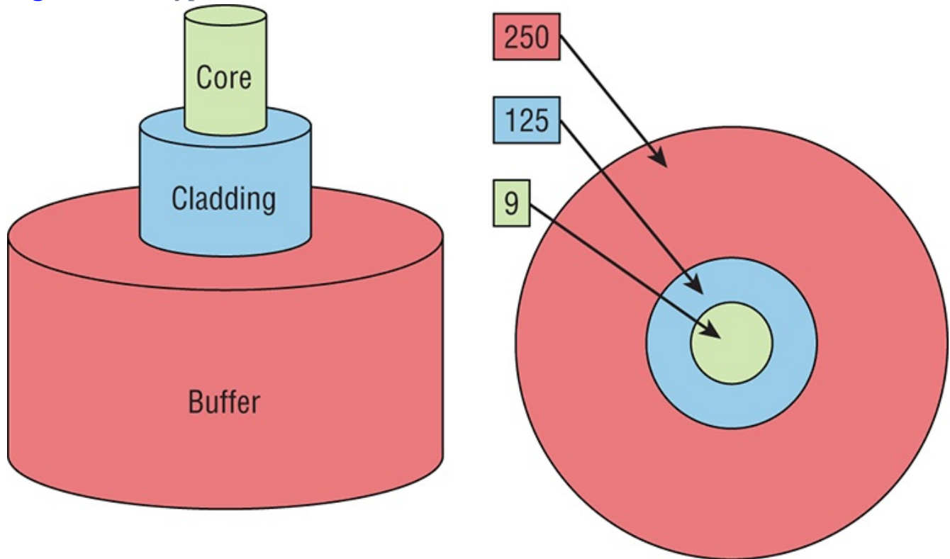
Figure 2-19: Typical fiber cable
