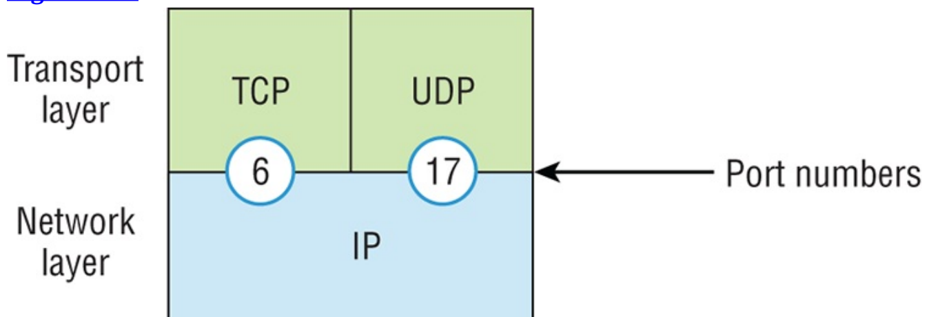
Figure 3-16: The Protocol field in an IP header
