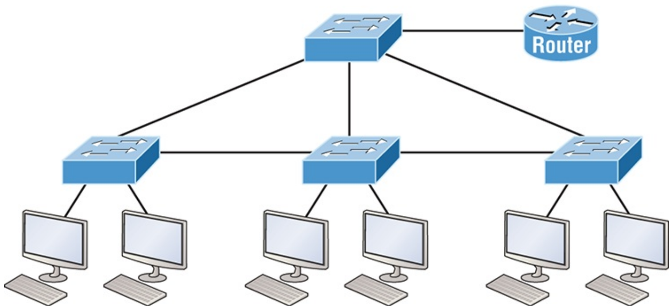
Figure 1-5: Switched networks creating an internetwork
