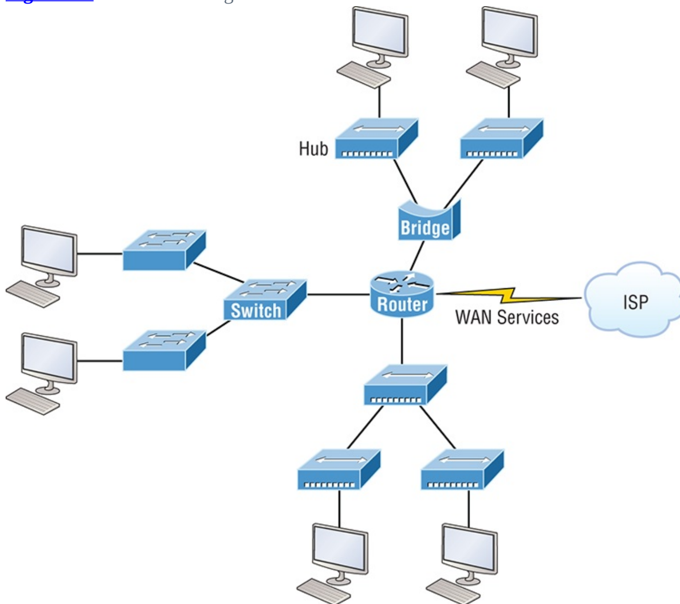
Figure 1-4: Internetworking devices
