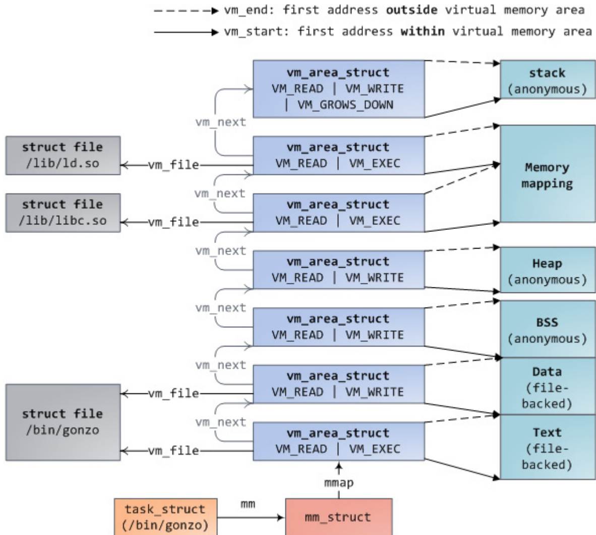
Figure 10.4 – Process memory mappings
