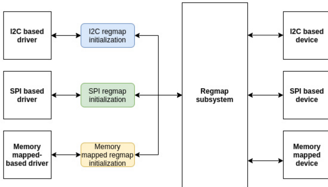
Figure 12.2 - I2C, SPI, and memory-mapped access after Regmap
