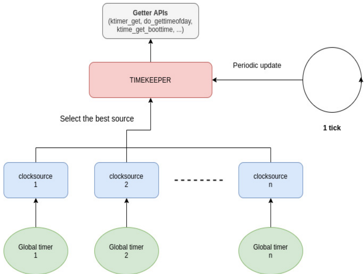
Figure 3.2 – Linux kernel timekeeper implementation
