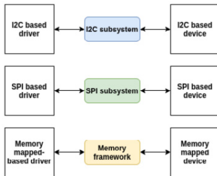
Figure 12.1 – I2C, SPI, and memory-mapped access before Regmap
