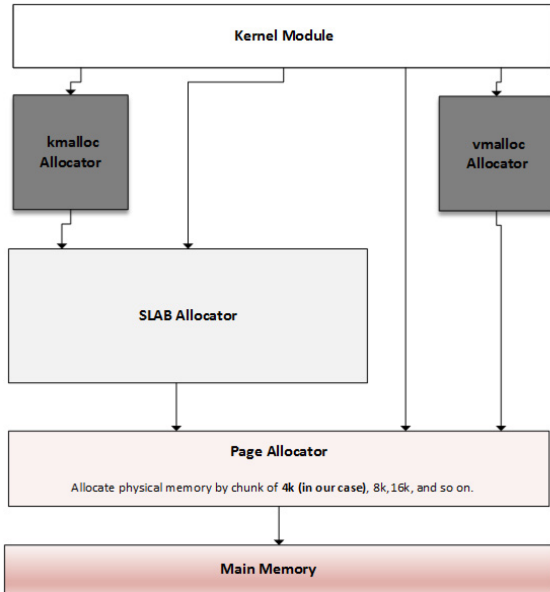
Figure 10.10 – Overview of kernel memory allocators
