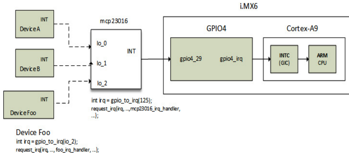
Figure 16.1 – Multiplexing IRQs
