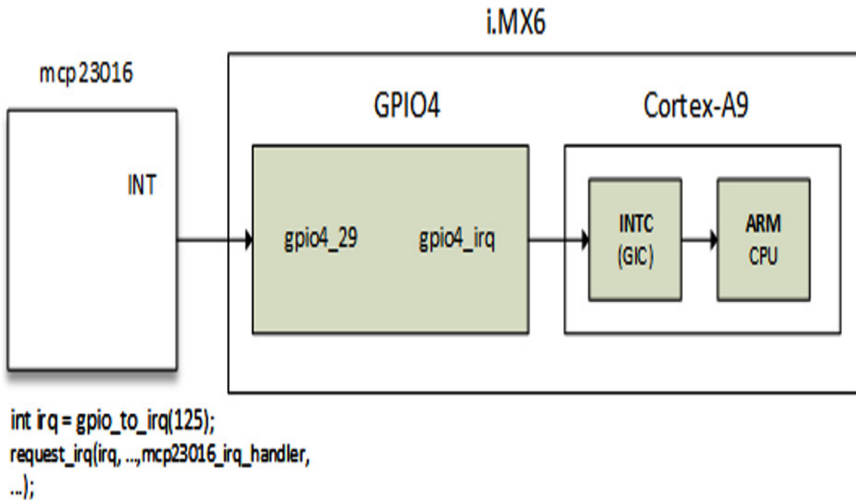
Figure 13.2 – Interrupt propagation
