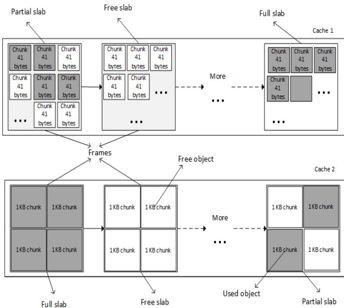
Figure 10.13 – Slabs and caches
