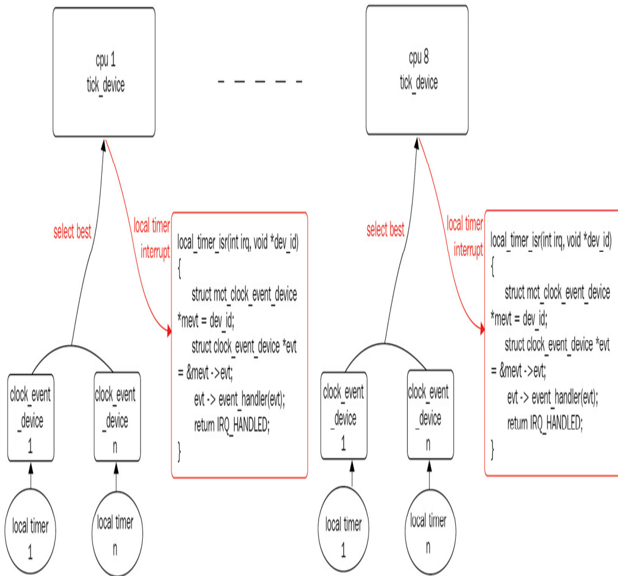
Figure 3.3 – Clockevent and tick-device correlation
