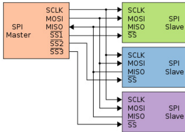
Figure 9.1 – SPI slave devices and master interconnection
