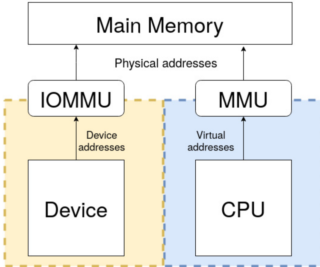
Figure 10.16 – (IO)MMU and main memory overview
