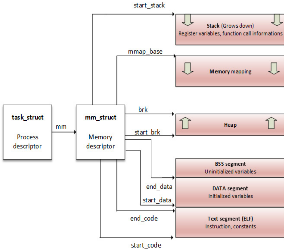
Figure 10.3 – A process address space
