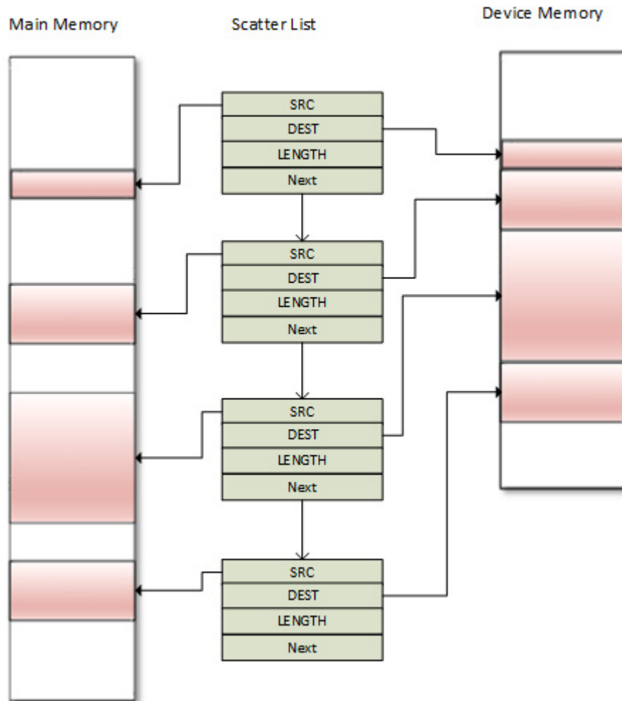
Figure 11.1 – Scatter/gather memory organization
