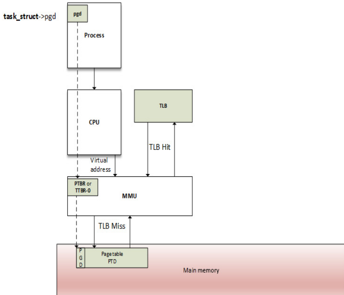
Figure 10.9 – The MMU and TLB walk-through process
