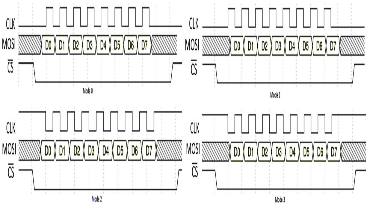
Figure 9.2 – SPI operating modes
