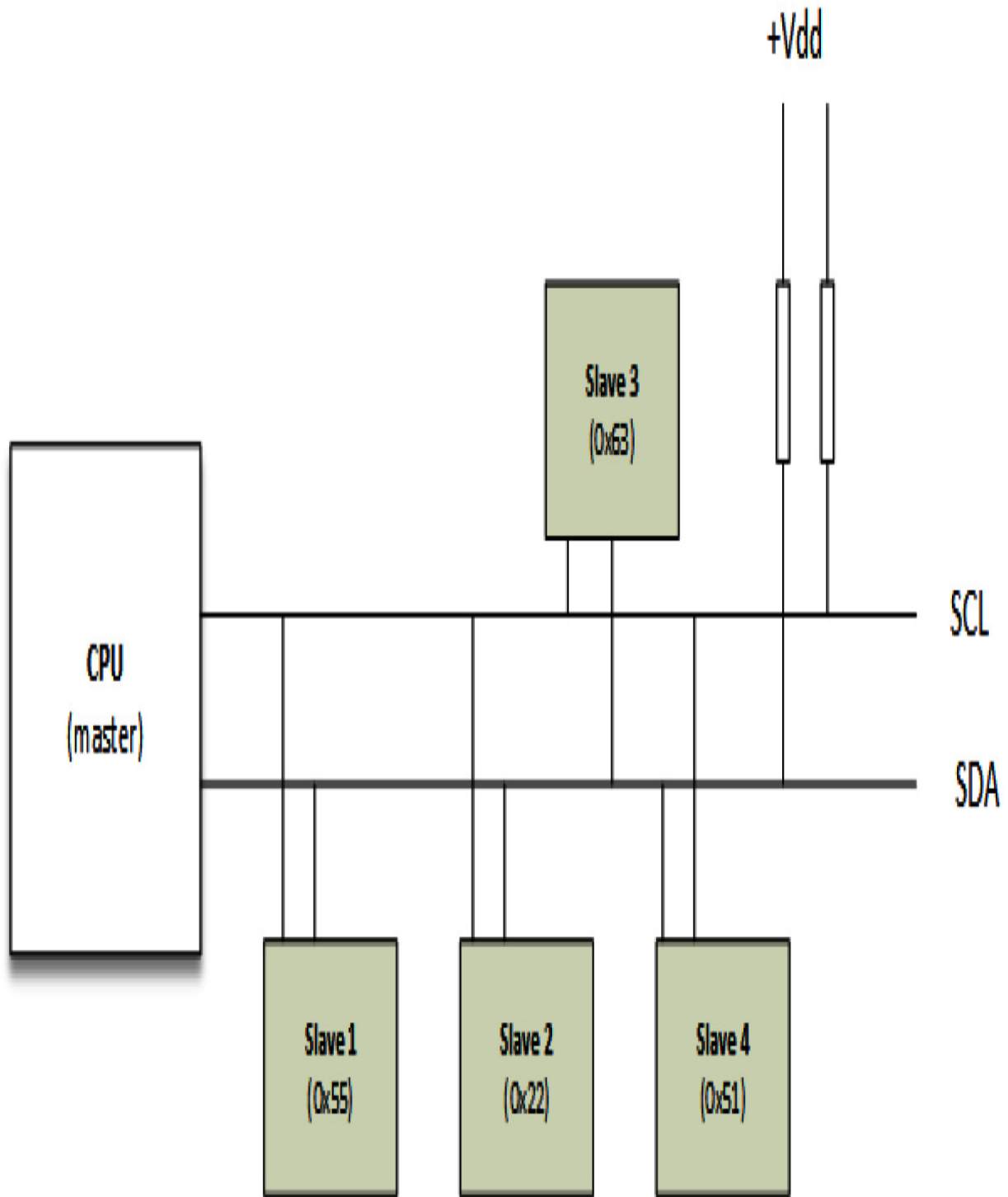
Figure 8.1 – I2C bus and device representation
