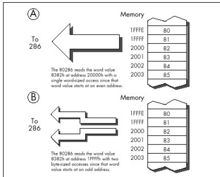
Figure 11.1 The data alignment cycle-eater.
