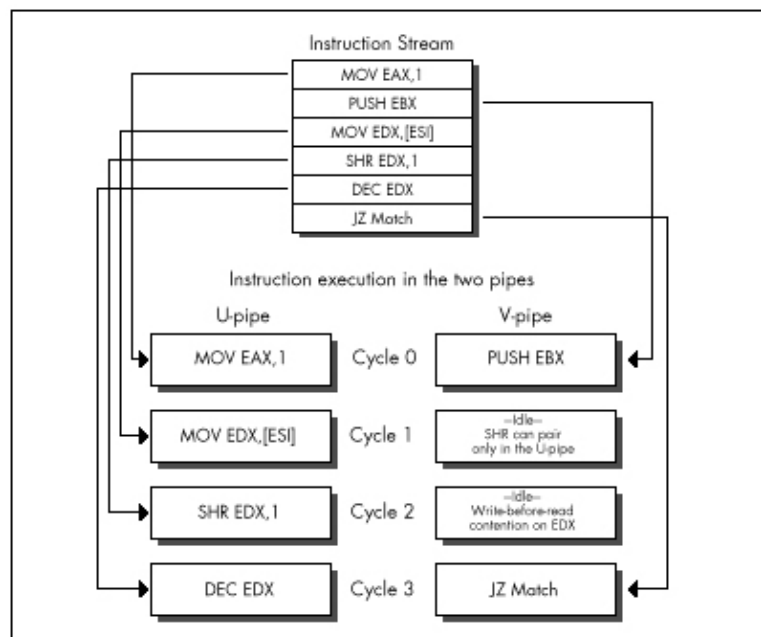
Figure 20.1 The Pentium's two pipes.
