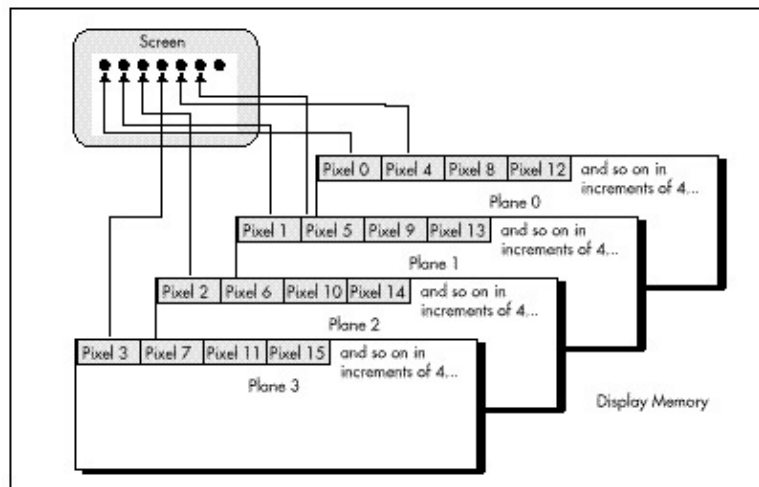
Figure 47.1 Mode X display memory organization.
