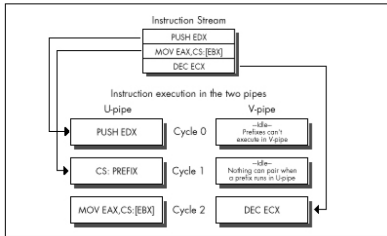
Figure 20.8 Prefix delays.
