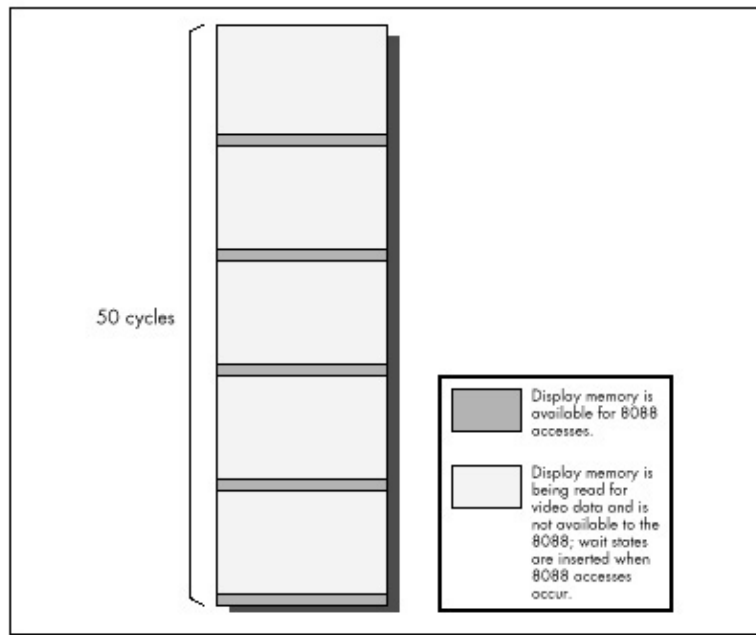
Figure 4.7 Allocation of display memory access.
