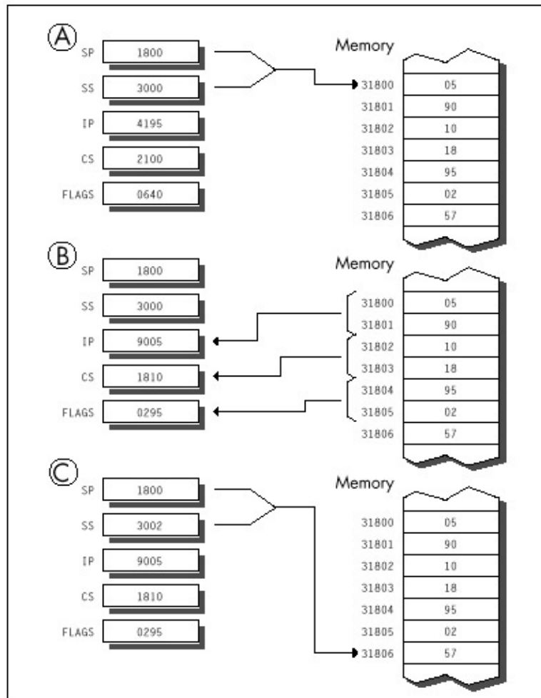
Figure 11.5 The operation of IRET.
