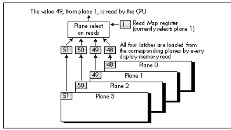
Figure 48.1 How the VGA latches are loaded.
