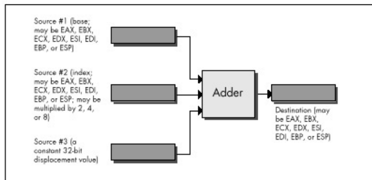
Figure 6.2 Operation of the 32-bit LEA reg,[Addr].
