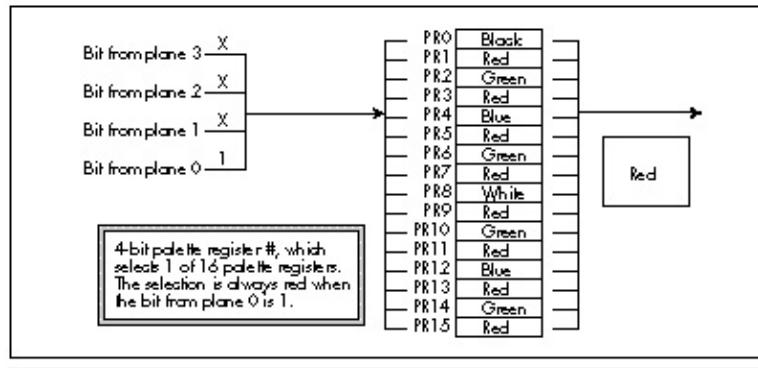
Figure 43.4 How pixel precedence works.
