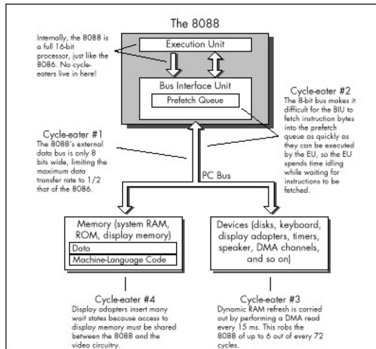
Figure 4.1 The location of the major cycle-eaters in the IBM PC.
