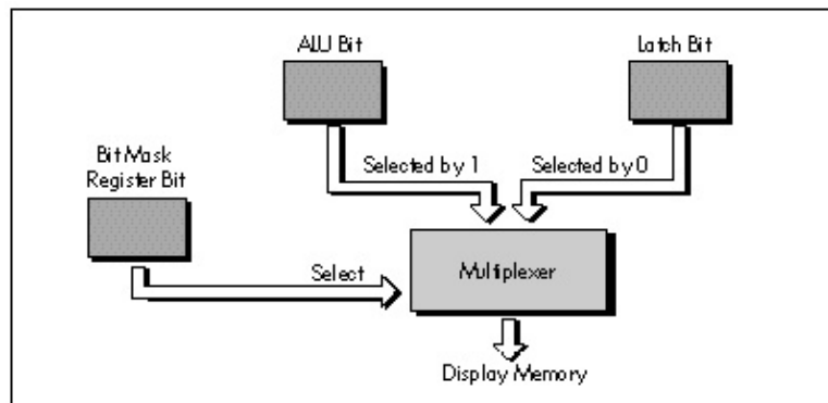
Figure 25.2 Bit mask operation.
