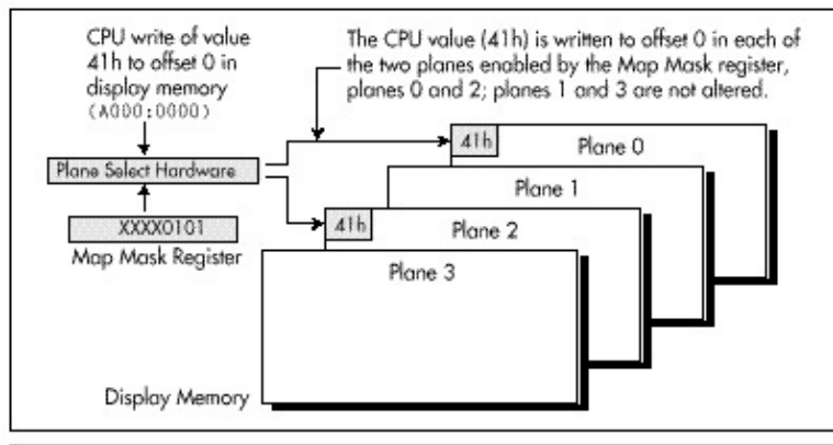
Figure 47.2 Selecting planes with the Map Mask register.
