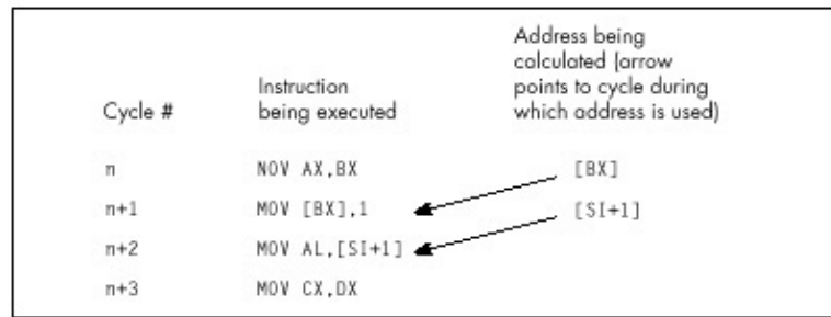
Figure 12.1 One-cycle-ahead address pipelining.
