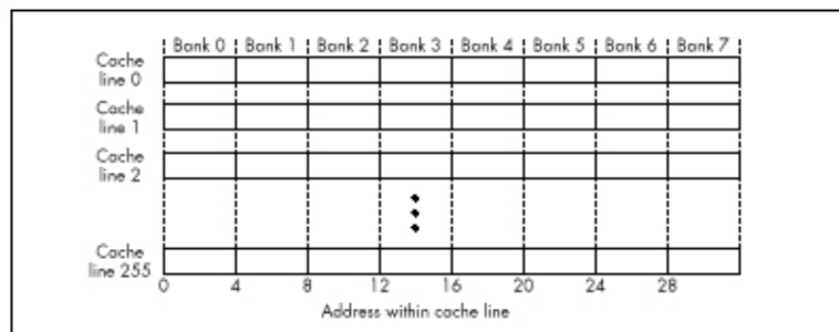
Figure 20.5 The Pentium's eight bank data cache.
