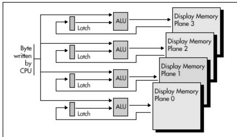
Figure 24.1 VGA ALU data flow.
