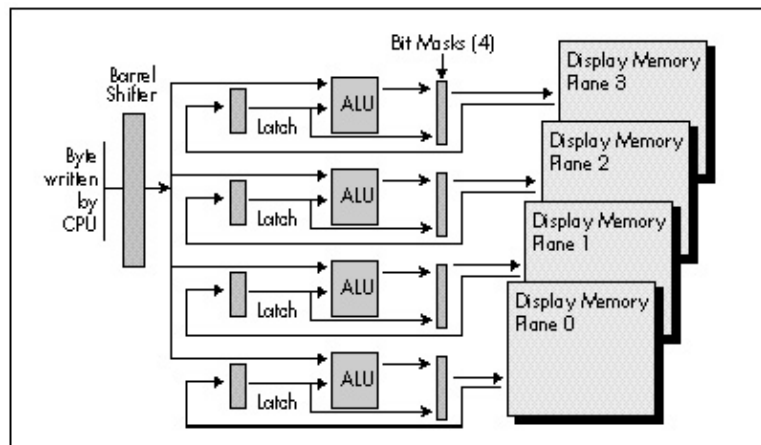
Figure 25.1 Data flow through the Graphics Controller.
