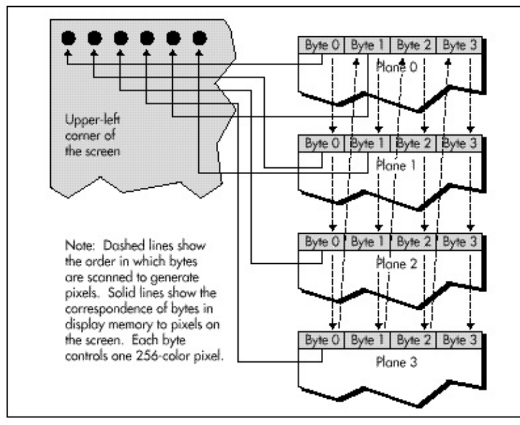
Figure 31.1 Bitmap organization in 320x400 256-color mode in 320x400 256-color
