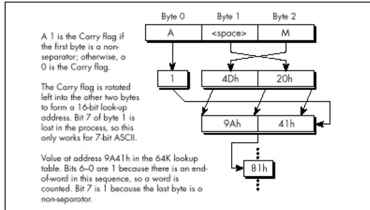
Figure 16.2 Looking up a word count status.
