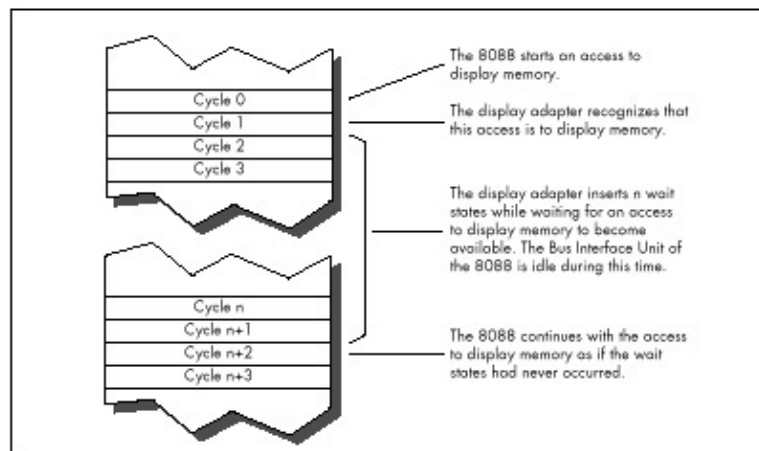
Figure 4.6 Video wait states inserted by the display adapter.
