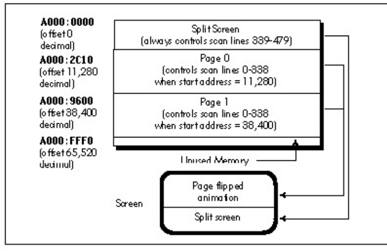
Figure 44.2 Memory allocation for mode 12h page flipping.
