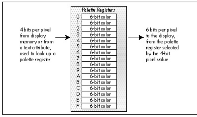
Figure 29.2 Color translation via the palette registers.
