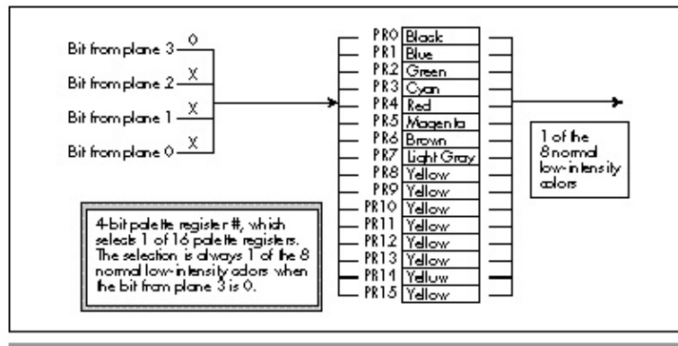
Figure 43.5 Pixel precedence for plane 3 only.
