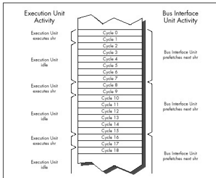
Figure 4.3 Execution and instruction prefetching sequence for Listing 4.5.
