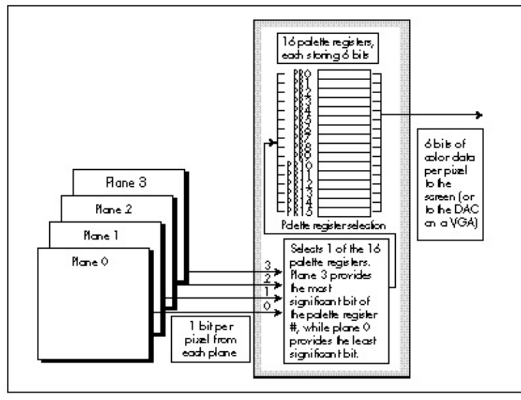
Figure 43.1 How 4 bits of video data become 6 bits of color.
