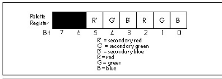
Figure 29.3 Bit organization within a palette register.
