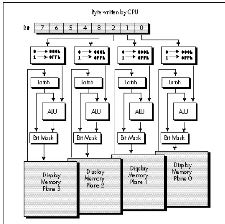
Figure 27.1 VGA data flow in write mode 2.
