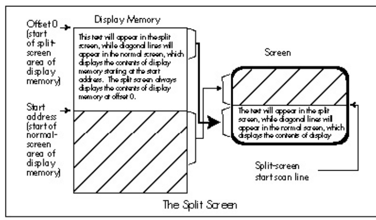
Figure 30.1 Display memory and the split screen.
