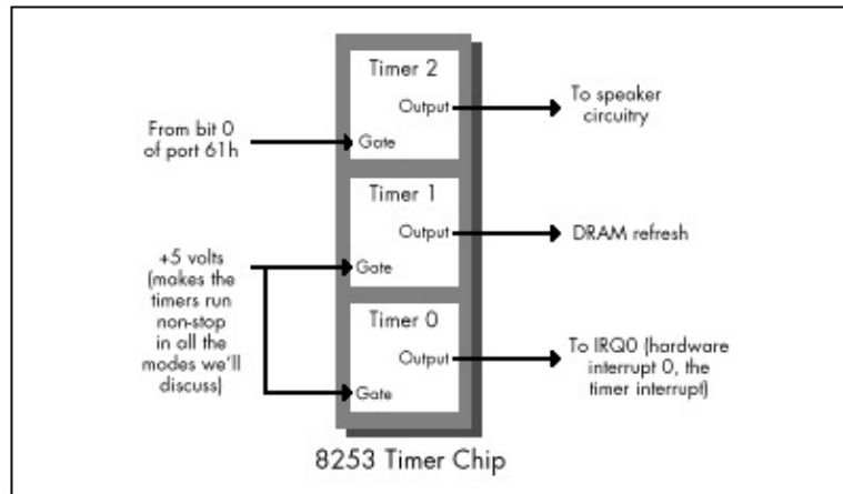
Figure 3.1 The configuration of the 8253 timer chip in the PC.
