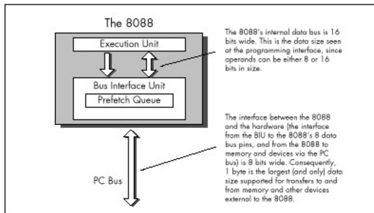
Figure 4.2 Internal data bus widths of the 8088.
