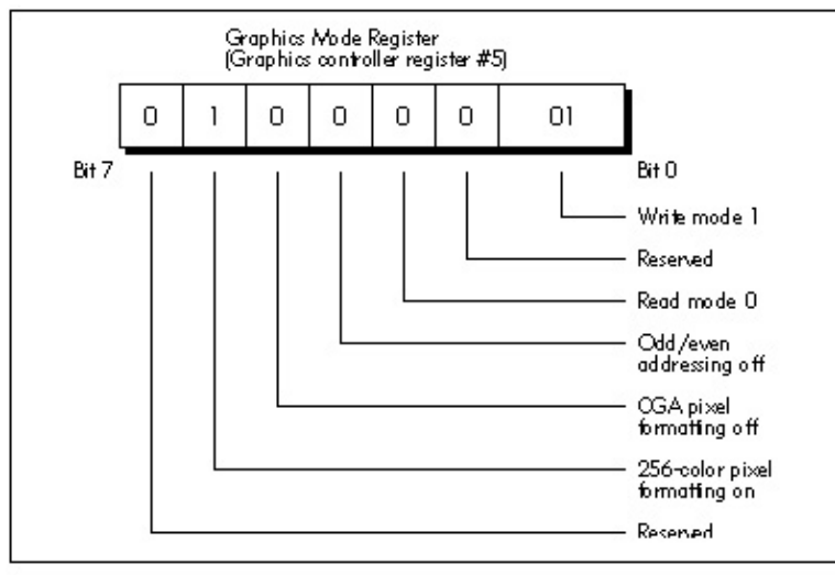
Figure 29.4 Graphics mode register fields.
