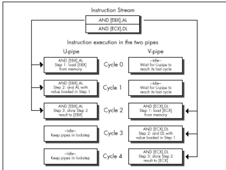
Figure 20.6 Non-overlapped lockstep execution.
