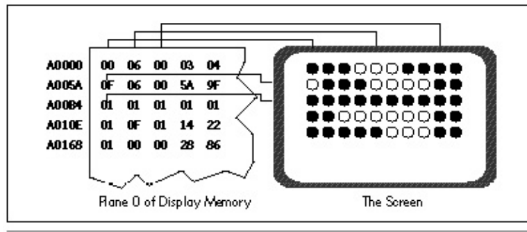
Figure 32.1 Pixel organization in 360x480 256-color mode.
