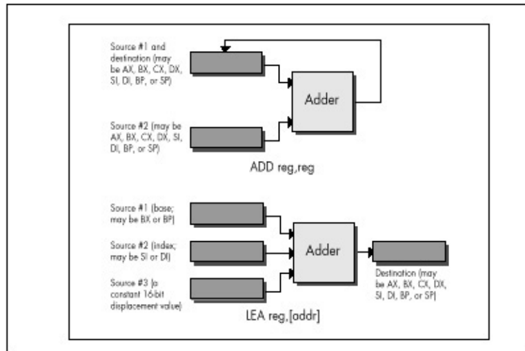
Figure 6.1 Operation of ADD Reg,Reg vs. LEA Reg,{Addr} .
