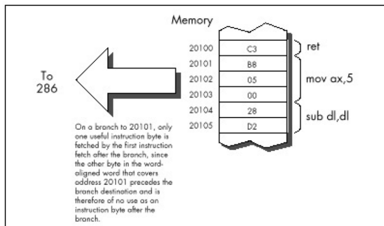
Figure 11.3 How instruction bytes are fetched after a branch.
