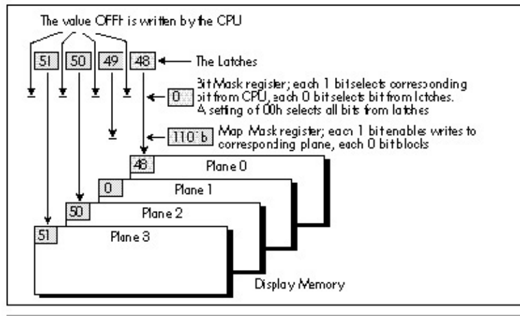
Figure 48.2 Writing 4 bytes to display memory in a single operation.
