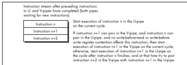
Figure 20.2 Instruction flow through the two pipes.
