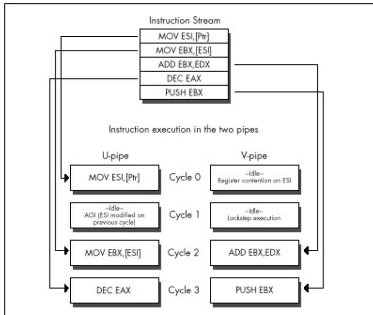
Figure 21.2 An AGI can cost as many as 3 cycles.
