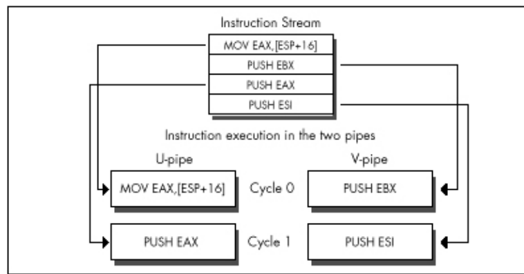
Figure 20.3 Pushing a value from memory effectively in one cycle.
