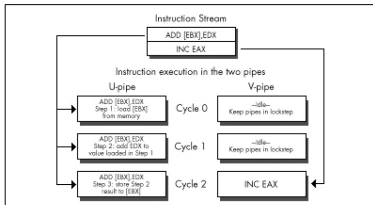
Figure 20.4 Lockstep execution and idle time in the V-pipe.
