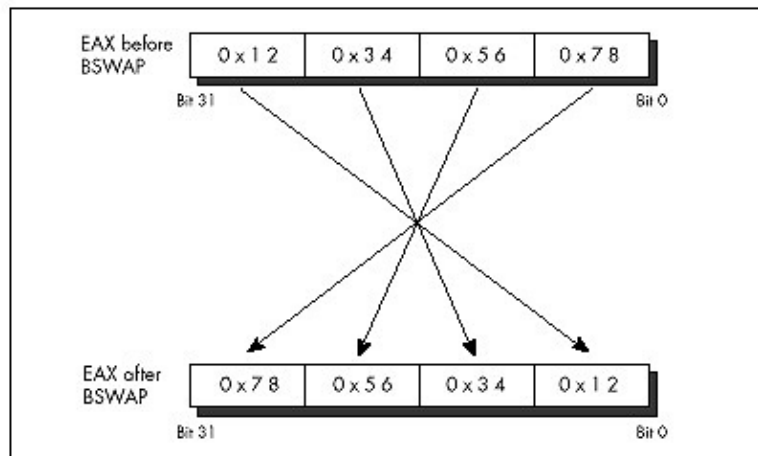
Figure 13.2 BSWAP in operation.
