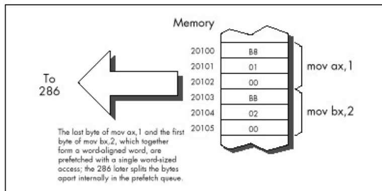
Figure 11.2 Word-aligned prefetching on the 286.
