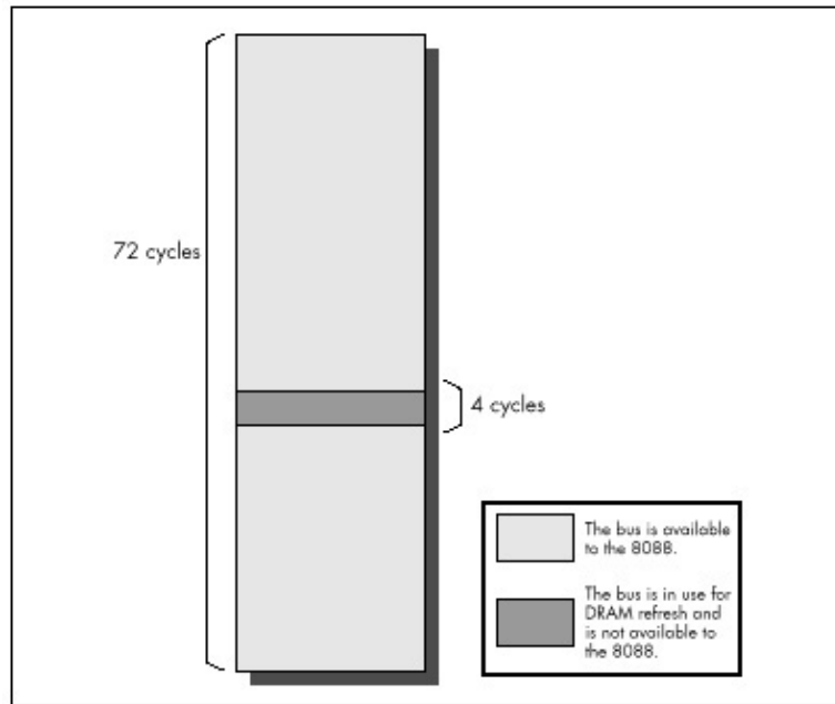
Figure 4.5 The PC bus dynamic RAM (DRAM) refresh.
