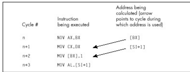
Figure 12.2 Two-cycle-ahead address pipelining.
