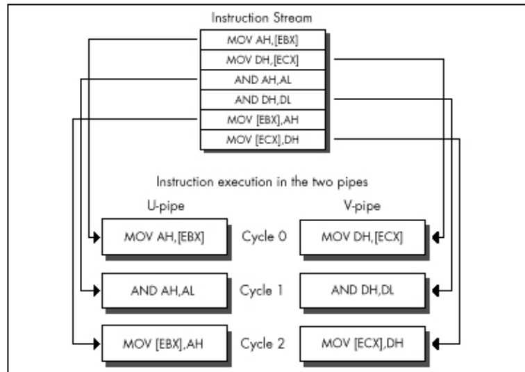
Figure 20.7 Interleaving simple instructions for maximum performance.
