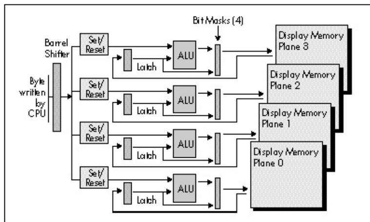
Figure 25.3 Data flow during a write mode 0 write operation.
