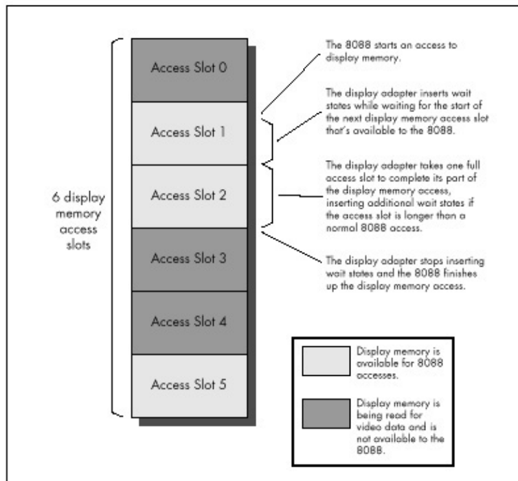
Figure 4.8 Display memory access slots.
