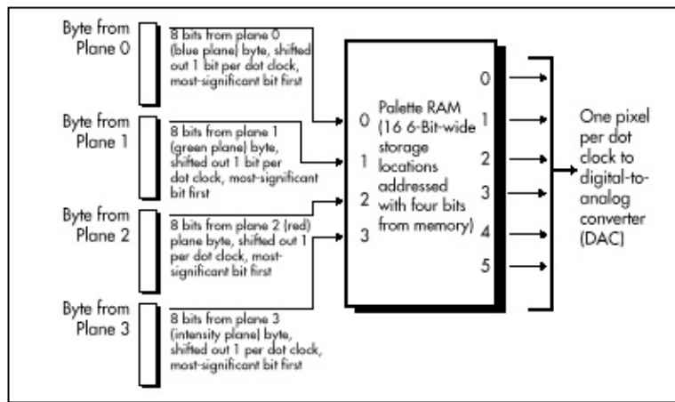
Figure 23.1 Video data from memory to pixel.
