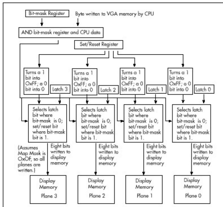
Figure 55.3 The data path in write mode 3.
