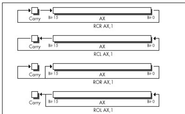
Figure 9.4 Performing rotate instructions using the Carry flag.
