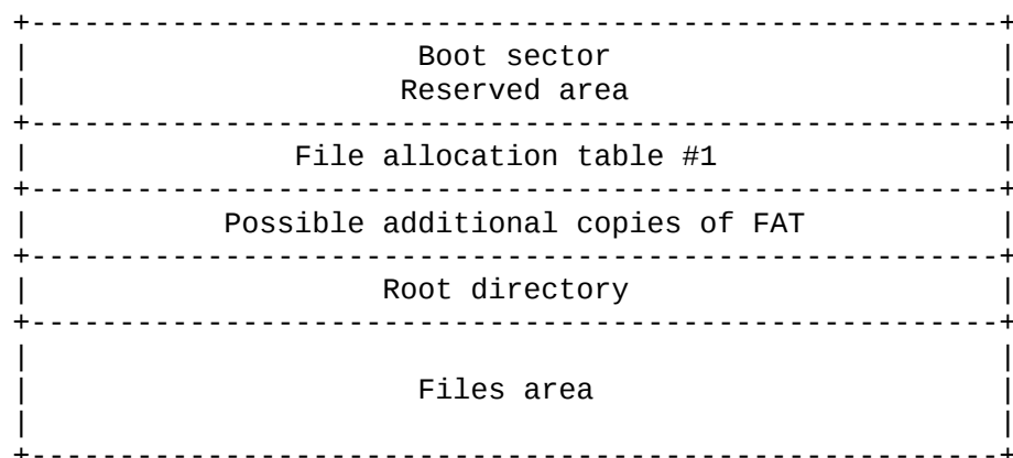
Figure 10-1. Map of a typical MS-DOS logical volume. The boot sector (logical sector 0) contains the OEM identification, BIOS parameter block (BPB), and disk bootstrap. The remaining sectors are divided among an optional reserved area, one or more copies of the file allocation table, the root directory, and the files area.
