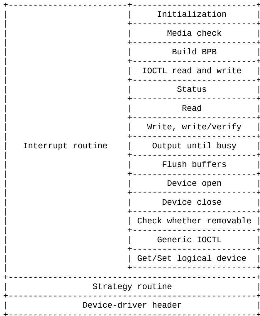
Figure 14-1. General structure of an MS-DOS installable device driver.
