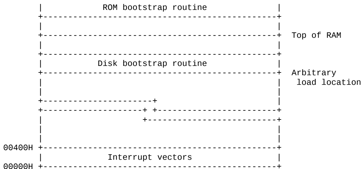
Figure 2-2. The ROM bootstrap routine loads the disk bootstrap routine into memory from the first sector of the system startup disk and then transfers control to it.
