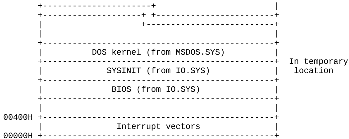
Figure 2-3. The disk bootstrap reads the file IO.SYS into memory. This file contains the MS-DOS BIOS (resident device drivers) and the SYSINIT module. Either the disk bootstrap or the BIOS (depending upon the manufacturer's implementation) then reads the DOS kernel into memory from the MSDOS.SYS file.
