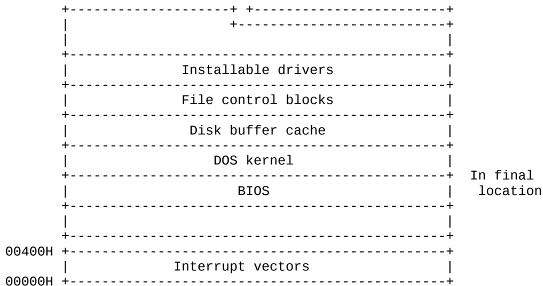
Figure 2-4. SYSINIT moves itself to high memory and relocates the DOS kernel, MSDOS.SYS, downward to its final address. The MS-DOS disk buffer cache and file control block areas are allocated, and then the installable device drivers specified in the CONFIG.SYS file are loaded and linked into the system.
