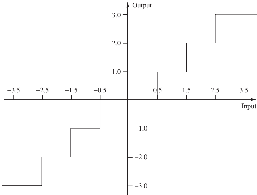
FIGURE 9.5 A midread quantizer.
