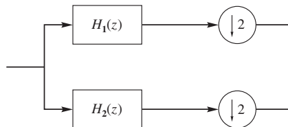
FIGURE 14.22 Analysis portion of a two-band subband coder.
