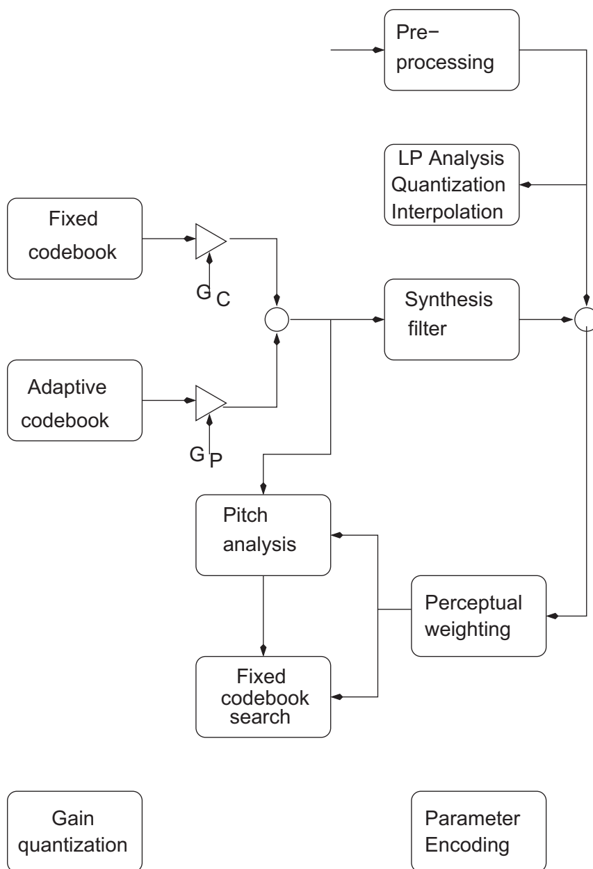
FIGURE 18.11 Steps in the encoding of speech for the ITU-T G.729 encoder.
